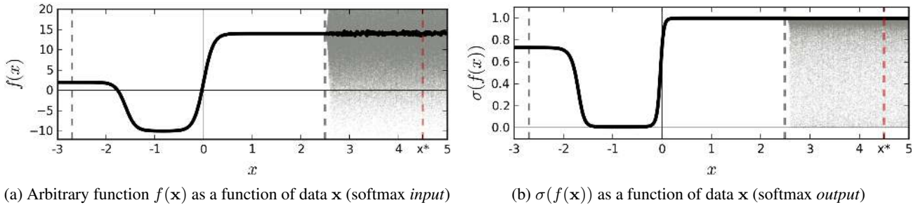
(a) Arbitrary function f(x) as a function of data x (softmax input)
