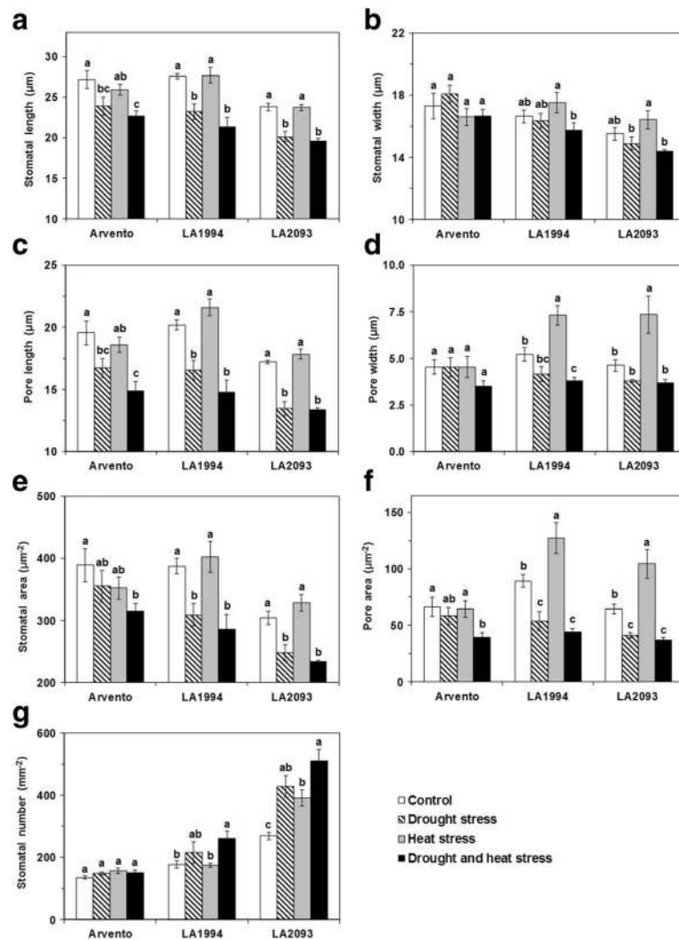
Fig. 5 Stomatal characteristics in the abaxial leaves of the three tomato cultivars under four days of control, drought, heat and combined stress. Different sub-graphs represent a stomatal length, b stomatal width, c pore length, d pore width, e stomatal area, f pore area and g stomatal number. The data represent mean values \pm SE ( n = 4 ). Different small letters above the bars indicate significant differences ( P < 0.05 )
