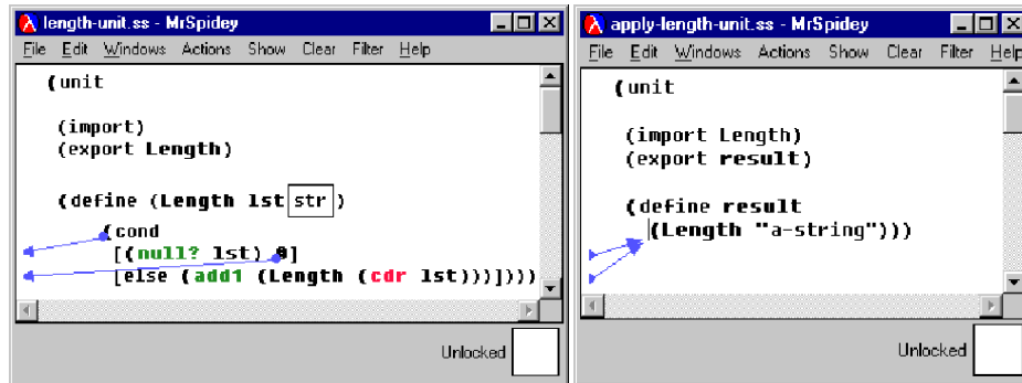
Figure 11. Analyzing multiple units in MrSpidey (Windows version).
