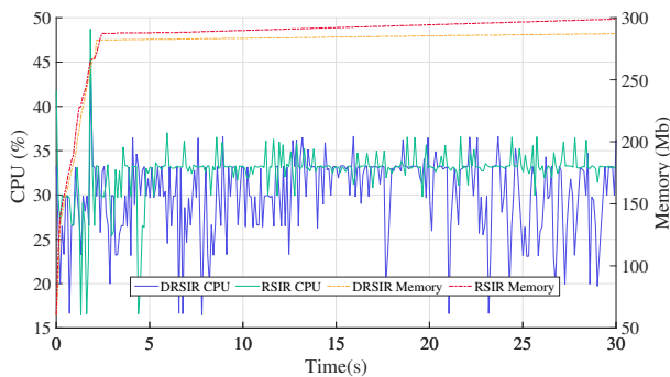
Fig. 5: CPU and Memory used by the agents of DRSIR and RSIR
