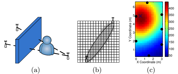
Figure 1: (a) A person blocks two radio links, creating a NLOS environment. (b) The AoI is divided into voxels. An ellipse is used to model the area of obstruction between a pair of nodes. (c) An example of an RTI image. The blue cross indicates the truth location of the obstruction. (Best view in colour.)
