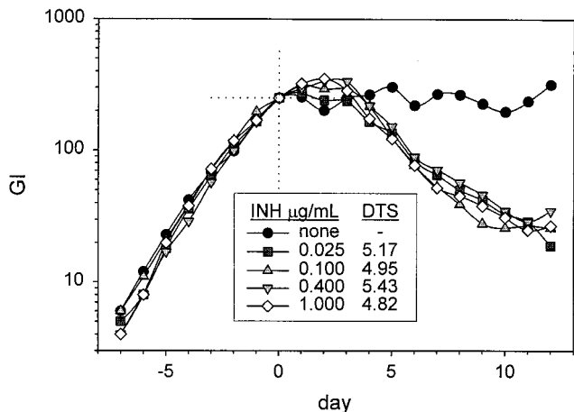
FIG. 6. Lack of effect of INH concentration on the rate of killing of a tolerant clinical M. tuberculosis isolate. All concentrations tested were greater than the MIC for this isolate.
