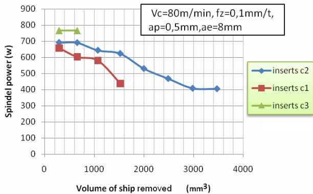
Fig. 11 Dependence Spindle Power consumption on volume of chip removed for three inserts ( V_c = 80 m/min, f_z = 0.1 mm/t)
