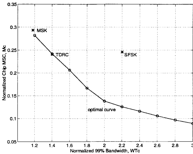
Fig. 5. Optimal performance limit (99% bandwidth measure) with continuous-phase and nonuniform envelope.
