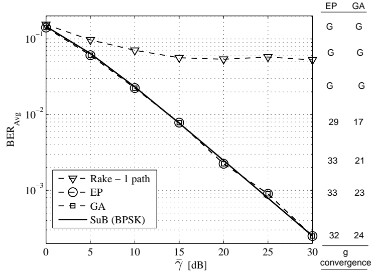
Figure 5: BER of system \mathbf{S}_1 , PD-3 profile and NFR = 0 dB.
