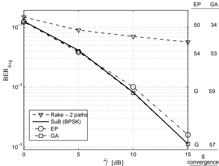
Figure 10: BER for the system \mathbf{S}_2 , NFR = 0 dB, PD-2 profile and D = L = 2 .
