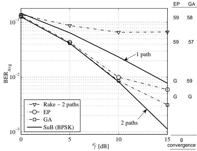
Figure 9: BER for the system \mathbf{S}_2 , NFR = 0\text{ dB} , PD-2 profile with D < L = 2 occasionally.
