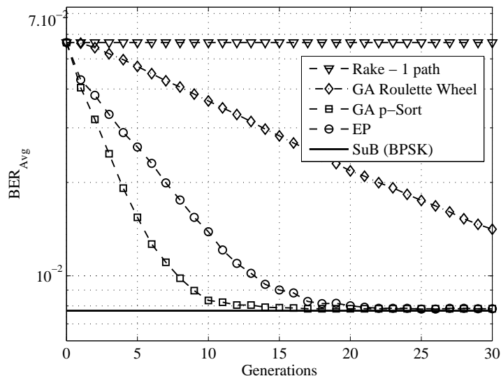
Figure 4: Convergence velocity for EP-MuD and GA-MuD; two selection strategies for the GA-MuD ( p -Sort and Roulette Wheel); System S_1 ; PD-3 profile; \bar{\gamma}_1 = 15 \text{ dB} and NFR = 0 \text{ dB} .
