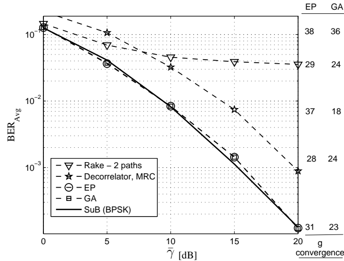
Figure 6: BER for the system \mathbf{S}_1 , NFR = 0 dB, PD-2 profile and D = L = 2 .
