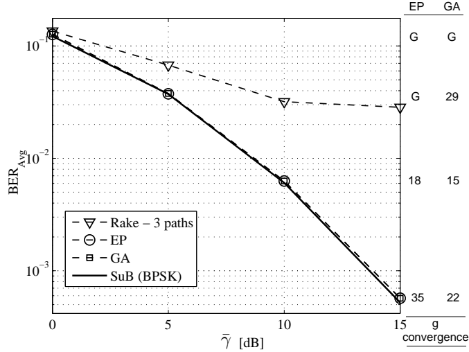
Figure 7: BER for the system S_1 , NFR = 0 dB, PD-1 profile and D = L = 3 .
