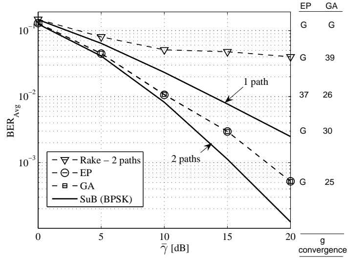
Figure 8: BER for the system \mathbf{S}_1 , NFR = 0\text{ dB} , PD-2 profile with D < L = 2 occasionally.
