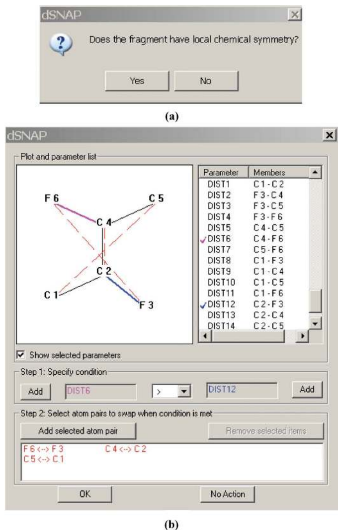
Figure 2 The initial dialog boxes that question the user about local chemical symmetry. The interface allows the user to define the necessary rules to ensure optimal clustering.
