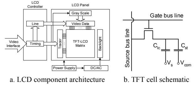
Figure 3. TFT-LCD screen
