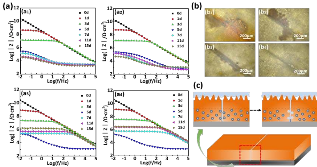
Fig. 7 (a) The evolution of Bode plots of healed superhydrophobic coatings immersed in a 3.5% NaCl solution for 15 days: (a 1 ) the BTAs-free coating, (a 2 ) the BTAs-1% coating, (a 3 ) the BTAs-3% coating and (a 4 ) the BTAs-5% coating. (b) The optical micrographs of healed superhydrophobic coatings taken after 15 days of immersion: (b 1 ) the BTAs-free coating, (b 2 ) the BTAs-1% coating, (b 3 ) the BTAs-3% coating and (b 4 ) the BTAs-5% coating. (c) Schematic of the anticorrosion mechanism of the healed superhydrophobic coatings.
