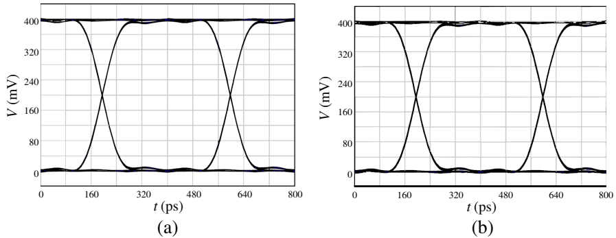
Figure 6. Measured differential eye diagrams for (a) a conventional pair of coupled lines (without etching in the ground plane) and (b) for the structure proposed in this paper.
