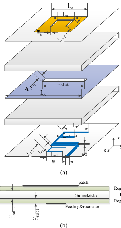
Fig.1. Configuration of the proposed dual-band filtering antenna: (a) exploded perspective view, (b) the stacked structure.
