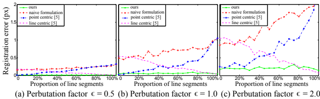
Figure 7. Comparisons of registration error between our formulation and others. Best viewed on screen.
