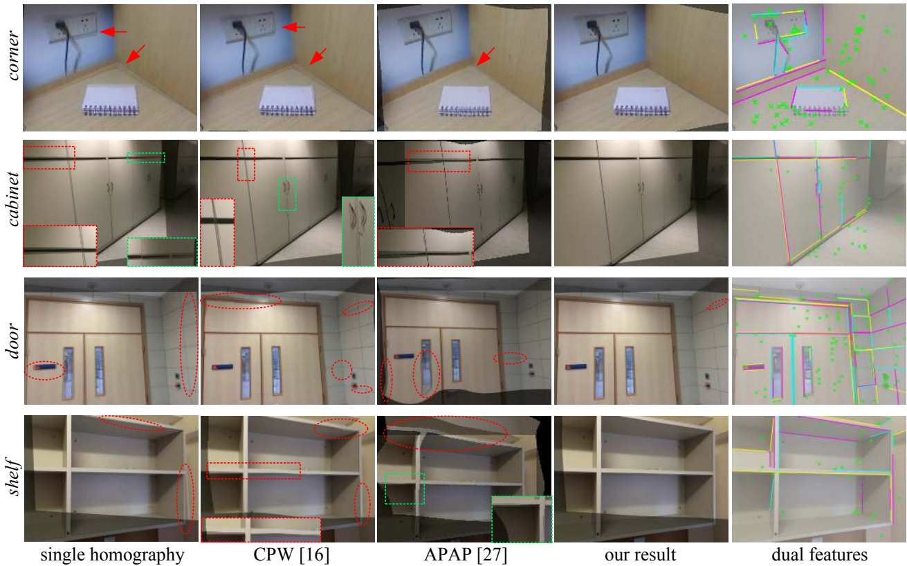
Figure 10. Comparison of image stitching on four image pairs from typical indoor scenes (best viewed on high-resolution digital display).
