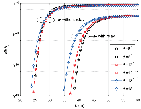
Fig. 8. Effect of the relay node on BER_t in coastal ocean for different beam divergence angles.
