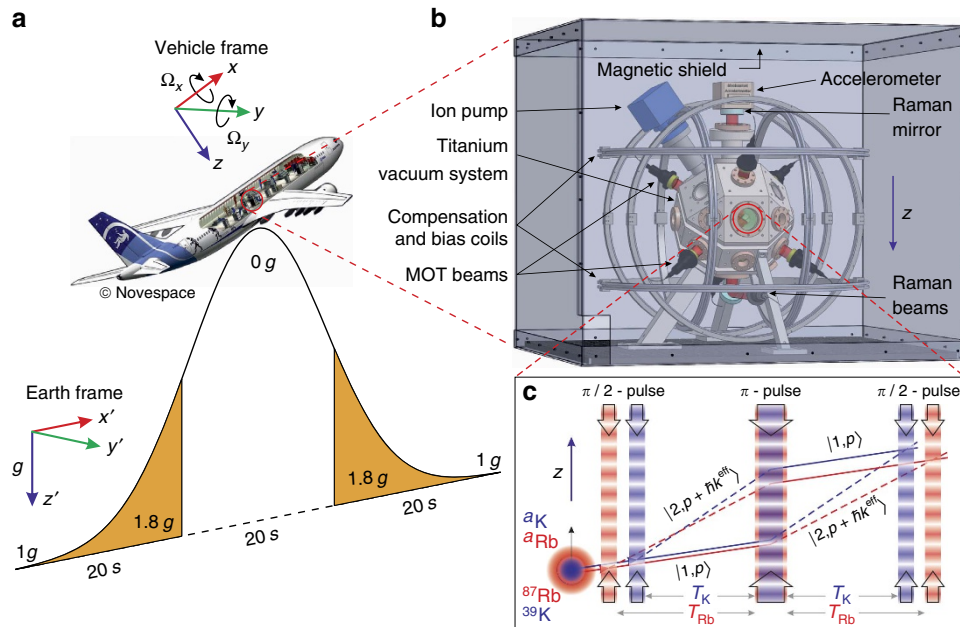
Figure 1 | Dual matter-wave sensors onboard the Novespace Zero-G aircraft. (a) Basic trajectory during parabolic flight, which produces 20 s of weightlessness per manoeuvre. The coordinate systems xyz and x'y'z' correspond to the rotating frame of the vehicle and the frame of the Earth, respectively. (b) The science chamber mounted onboard the aircraft. Samples of ^{87}\text{Rb} and ^{39}\text{K} are laser-cooled and spatially overlapped in a vapour-loaded magneto-optical trap contained within a titanium vacuum system, which is enclosed by a mu-metal magnetic shield. Raman beams are aligned along the z axis of the aircraft. (c) Schematic of the simultaneous dual-species interferometers. Two Mach-Zehnder-type \pi/2 - \pi - \pi/2 -pulse sequences are centred about the \pi -pulse with interrogation times T_{\text{Rb}} and T_{\text{Kr}} , respectively. These free-fall times are adjusted independently to equilibrate the scale factors of each interferometer.
