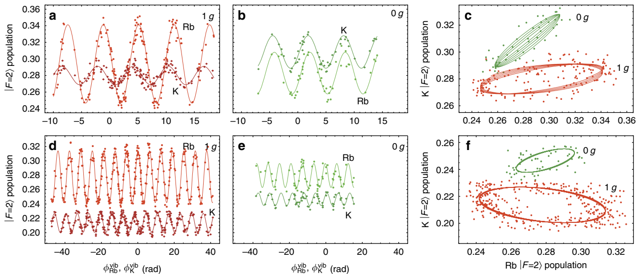
Figure 3 | Simultaneous K-Rb interferometer fringes during standard- and microgravity. The normalized population in the ground-state |F=2\rangle for each species is correlated with the vibration-induced phase \phi^{\text{vib}} for an interrogation time T \approx 1 ms ( a-c ) and T \approx 2 ms ( d-f ). Fringes labelled 0g were recorded over three consecutive parabolas for b , and five parabolas for e , consisting of \sim 12 points per parabola. Fringes labelled 1g were recorded during periods of steady flight between parabolas, and consist of \sim 70 points per manoeuvre. In a,b,d and e , solid lines indicate least-squares fits to sinusoidal functions, which yield a typical SNR of 7 for ^{87}\text{Rb} and 5 for ^{39}\text{K} data. ( c,f ) Correlations between population measurements for each interferometer. The solid lines are parametric representations of the corresponding fit functions shown in a,b,d and e . The interferometer scale factor ratio was computed using \kappa = S_K/S_{\text{Rb}} , where S_j = k_j^{\text{eff}}(T_j + \tau_j^\pi)(T_j + 2\tau_j^\pi/\pi) is the exact scale factor for species j (ref. 25). This yielded \kappa \approx 0.985 for a-c and \kappa \approx 1.001 for d-f . Other parameters: ( a-c ) T_{\text{Rb}} = 1.01 ms, T_{\text{K}} = 1 ms; ( d-f ) T_{\text{Rb}} = 2.01 ms, T_{\text{K}} = 2 ms; ( a-f ) \pi -pulse durations: \tau_{\text{Rb}}^\pi = 17 \mu\text{s} , \tau_{\text{K}}^\pi = 9 \mu\text{s} .
