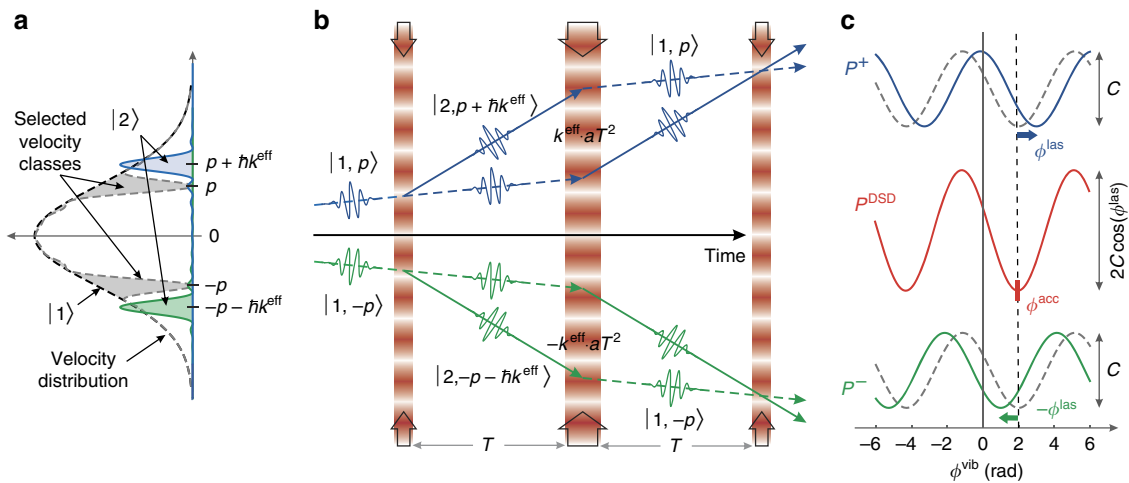
Figure 2 | Principles of the DSD interferometer. (a) Velocity distribution of the atoms in microgravity. The Raman frequency is tuned near the half-maximum—simultaneously selecting two symmetric velocity classes with opposite signs. (b) DSD interferometer trajectories. Double Raman diffraction 43 is avoided by ensuring that the Rabi frequency is much less than the Doppler frequency difference ( P^\pm ) between the two selected velocities. (c) Interference fringes as a function of the vibration phase \phi^{\text{vib}} for upward and downward interferometers ( P^\pm ) and the sum of the two ( P^{\text{DSD}} ). Direction-independent phase shifts like the laser phase \phi^{\text{las}} modulate the contrast but not the phase of the DSD fringes (other phase contributions have been omitted for simplicity).
