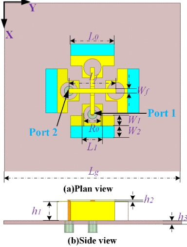
Fig. 5. Configuration of the proposed antenna unit: (a) Plan view; (b) Side view.
