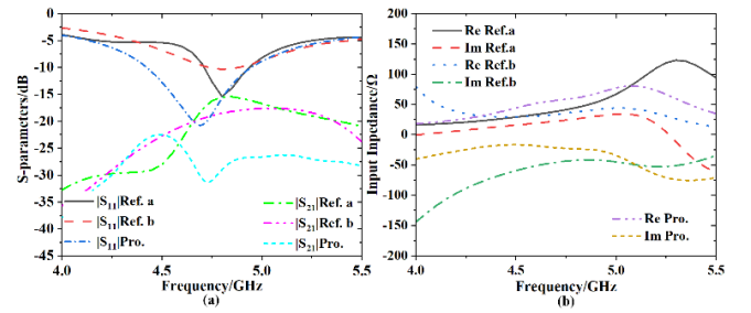
Fig. 6. (a) S -parameters and (b) input impedance of three antenna units.
