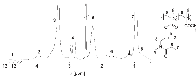
Figure 2. ^1\text{H} NMR spectra (250 MHz, \text{DMSO}-d_6 ) of P2 and assignment of the proton signals to the schematic representation of the polymeric structure.
