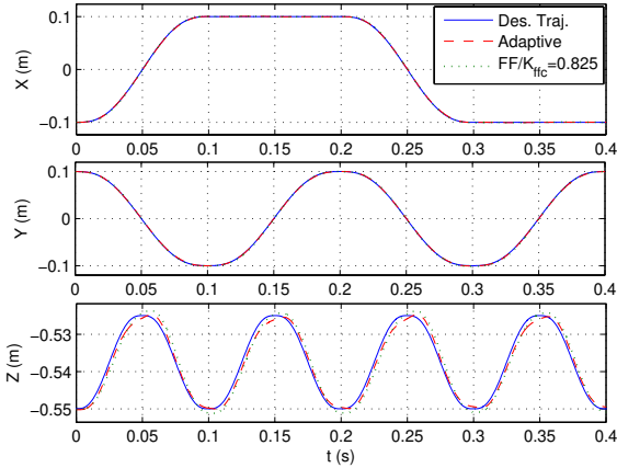
Fig. 24. 3D pick-and-place trajectory tracking with a payload of 200g for 1 cycle and an acceleration of 20G
