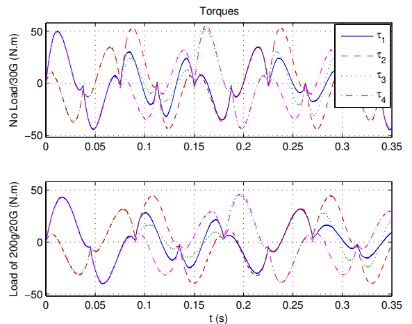
Fig. 23. Evolution of torques vs. time generated by the proposed dual-space feedforward controller
