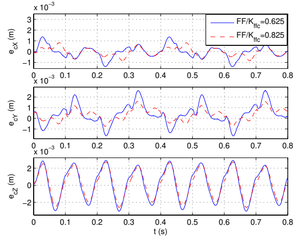
Fig. 22. Tracking errors for 20G with load, with different values of K_{ffc}
