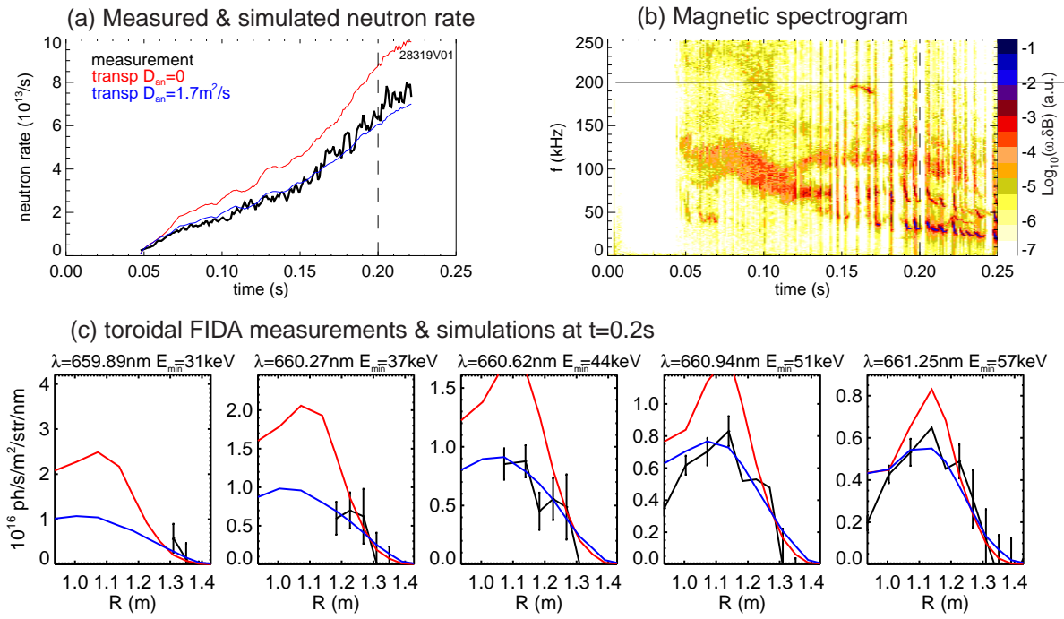
FIG. 14: Comparison of measured fast ion data with simulations in #28319. (a) Time history of neutron rate and simulation assuming various diffusion models. (b) Magnetic spectrogram showing presence of fishbones and other chirping mode activity. (c) Comparison of measurements with modelling considering different diffusion models late during the discharge (the colours corresponding to particular models are the same as those used in (a)).
