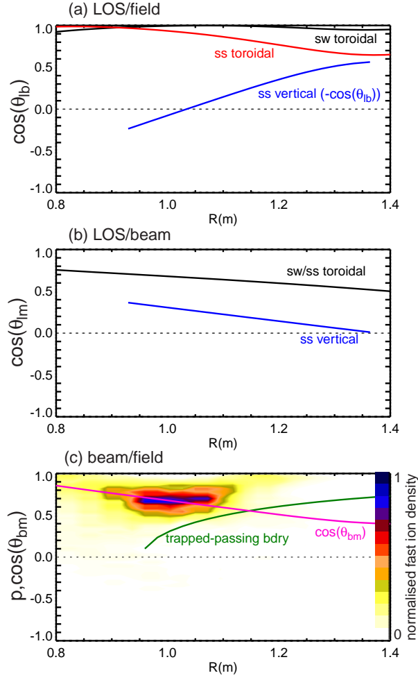
FIG. 2: (a) Cosine of angle between the line of sight and the magnetic field at the position of the beam for different views (the value on the SS vertical is inverted to compare blue shifted wavelengths with red shifted ones with the same value of E_{\min} ). (b) Cosine of angle between the beam and the line of sight, which determines the beam emission wavelengths. (c) Simulated TRANSP fast ion distribution (normalised) for MAST shot #26887 for E > 30keV as a function of (R, p) and birth pitch parameter \cos \theta_{bm} . (For this shot, B_t = 0.5T , I_p = 800kA .) The trapped-passing boundary [56] is shown for reference.
