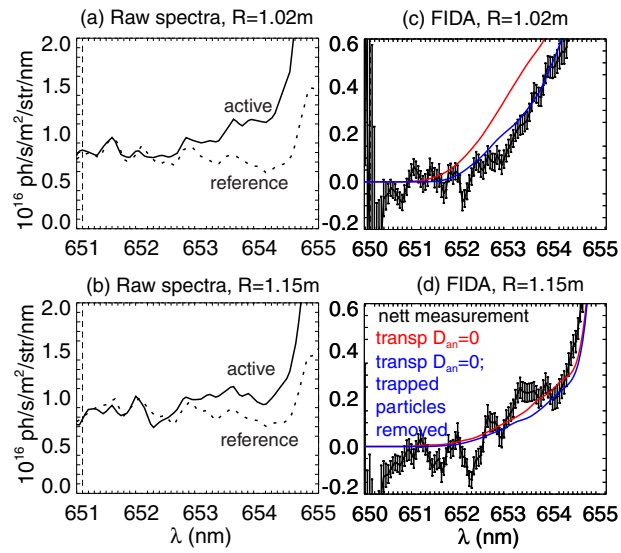
FIG. 12: Spectra at (a) inner and (b) outer radii on vertical channels for #26887, and (c, d) comparison of the net active FIDA signal with simulations.
