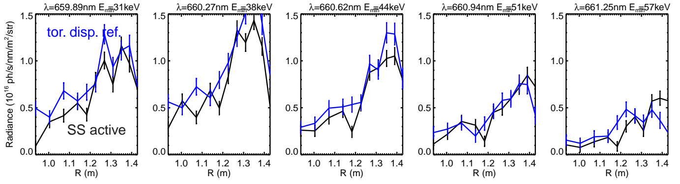
FIG. 9: Comparison of radial profiles of passive toroidal FIDA signals from the active view (installed on the downwards-directed SS view) derived just after the beam switch off and from the toroidally-displaced downwards-directed reference view, taken at t = 0.205\text{s} on #28322 (similar to chirping mode shot #28319 shown in Figure. (14)).
