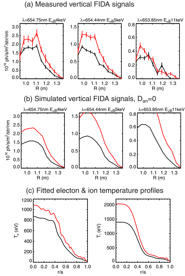
FIG. 13: (a) Comparison of low energy vertical FIDA signals between 1 (black) and 2 (red) beam shots #26887 (where neutron rate agrees with modelling assuming D_{an} = 0 ) and #26864 (neutron rate matched by D_{an} = 1.5m^2/s ). (b) Simulated FIDA profiles. (c) Electron and ion temperature profiles input to TRANSP
