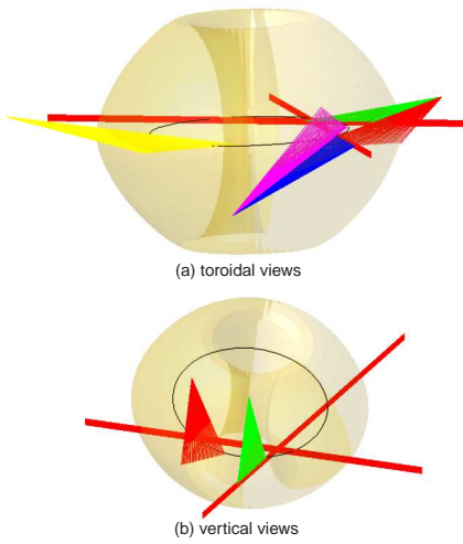
FIG. 1: 3D view of the sight lines of (a) toroidally-viewing chord bundles (blue: active on the SS beam, green: active on the SW beam, purple: vertically-displaced reference on the SW beam, red: vertically-displaced reference on the SS beam, yellow: toroidally-displaced reference) and (b) vertically-viewing chord bundles (green: active on the SS beam and red: toroidally-displaced reference view).
