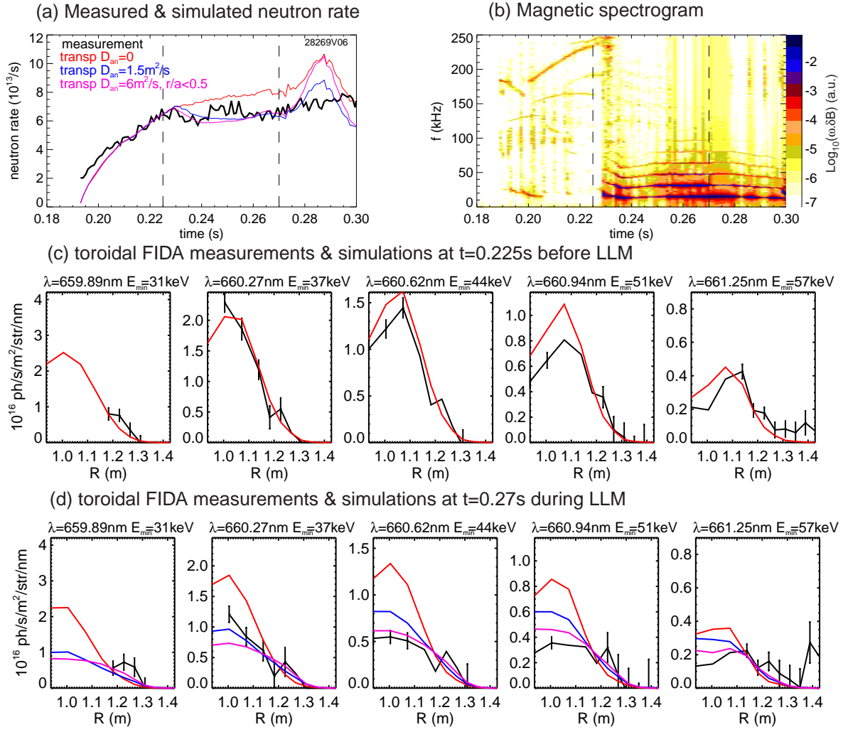
FIG. 10: Comparison of measured fast ion data with simulations in #28269. (a) Time trace of neutron rate and simulation assuming various diffusion models. (b) Magnetic spectrogram showing the onset of a LLM at 0.23s. (c) Toroidal FIDA measurements at different wavelengths and classical modelling during the quiescent phase. (d) Comparison of measurements with modelling considering different diffusion models during the LLM (the colours corresponding to particular models are the same as those used in (a)).
