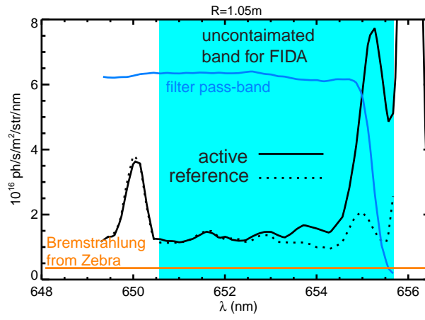
FIG. 6: Measured active and reference spectra for an inner channel of the vertical-viewing fibres, compared with the filter pass-band and the calculated bremsstrahlung background.
