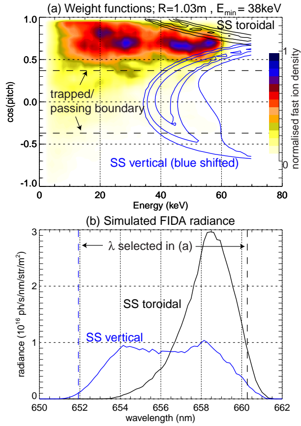
FIG. 3: (a) The TRANSP-simulated fast ion distribution (for shot #26887, t = 0.25\text{s} ) at R = 1.03\text{m} as a function of pitch and energy together with the approximate energy response functions at E_{\text{min}} = 38\text{keV} for the SS toroidal view ( \lambda = 660\text{nm} ) and vertical view ( \lambda = 652\text{nm} ). Horizontal dashed lines indicate the trapped/passing boundary. (b) FIDA radiance for the horizontal and vertical chords looking at R = 1.02\text{m} derived from the FIDASIM code for the same shot and time, indicating the wavelengths corresponding to the weight functions plotted in (a).
