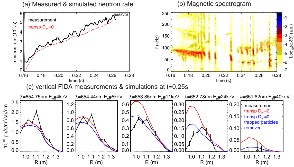
FIG. 11: Comparison of measured fast ion data with simulations in #26887. (a) Time history of neutron rate and classical simulation. (b) Magnetic spectrogram showing weak chirping activity. (c) Vertical FIDA measurements at different wavelengths (much lower energies than the toroidal ones) and modelling assuming classical transport and also considering an absence of trapped particles, to elucidate their contribution to the signal.
