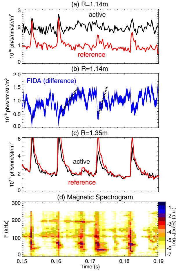
FIG. 15: Detailed analysis of toroidal FIDA signal evolution during shot #28319 at \lambda = 660.6\text{nm} ( E_{\min} = 44\text{keV} ) for a core (a,b) and edge (c) channel, comparing active channel (black) and passive channel (red) in (a,c) as well as the core net active FIDA signal (b), where the thickness of the line denotes the shot noise error bar. (d) Comparison with the magnetic spectrogram.
