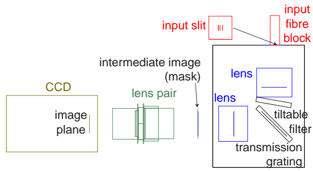
FIG. 4: Schematic of the spectrometer and CCD showing the fibre array, tiltable filter holder, grating, intermediate image location where masks can be inserted, second relay lens array and CCD.
