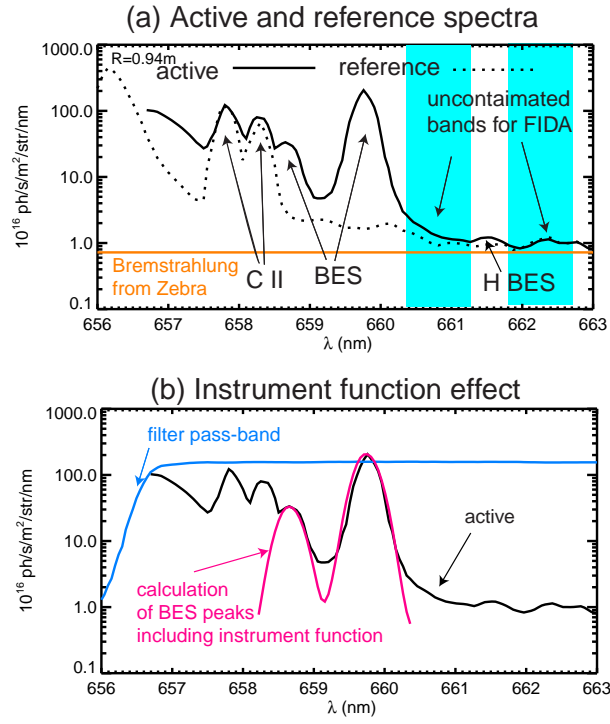
FIG. 5: (a) Active and (toroidally-displaced) reference spectra at R = 0.94\text{m} and computed bremsstrahlung background (scaled from Zebra diagnostic, considering wavelength difference), highlighting the uncontaminated spectral region available for FIDA: between the BES peak and the H BES peak; and above the H BES peak, which does not contain any FIDA at this radius, but does contain FIDA in edge channels. (b) Active spectra, compared with the synthesized BES peaks considering the measured instrument function width, as well as the filter pass-band.
