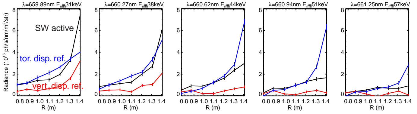
FIG. 8: Comparison of radial profiles of passive toroidal FIDA signals from the active view (installed on the upward-directed SW view) derived just after the beam switch off; from the toroidally-displaced, downwards-directed reference view; and from the vertically-displaced, upwards-looking reference view. Data are at t = 0.24\text{s} on #28141 (for which two reference views were simultaneously acquired).
