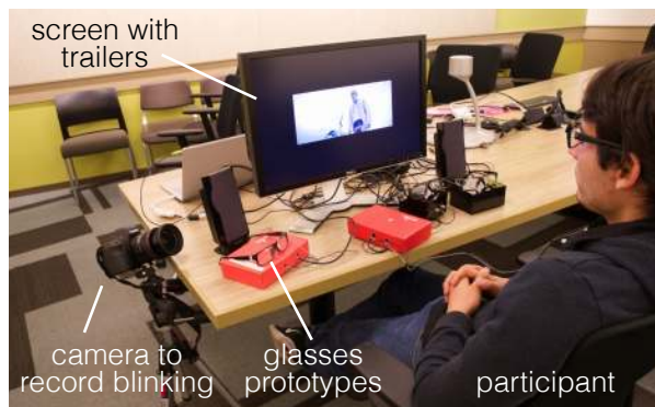
Fig. 7. The setup during the first and second setup. The participant watched trailers on the monitor while wearing each of the four prototype glasses.
