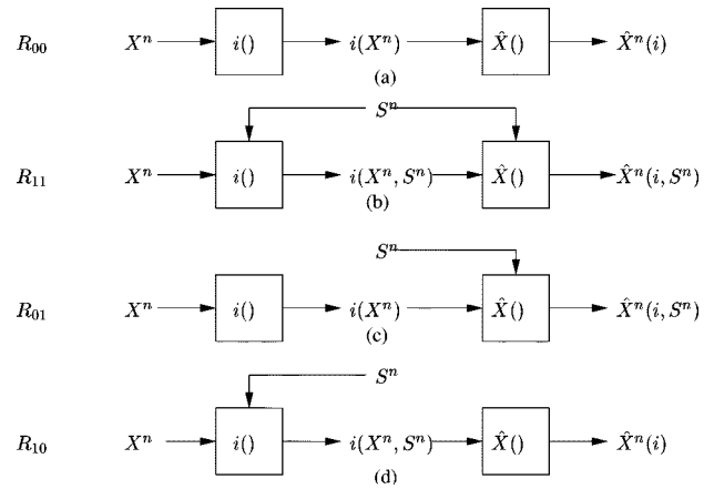
Fig. 2. Rate distortion with state information. Four special cases. (a) R_{00} = \min_{p(\hat{x}|x)} I(X; \hat{X}) . (b) R_{11} = \min_{p(\hat{x}|x,s)} I(X; \hat{X}|S) . (c) R_{01} = \min_{p(u|x)p(\hat{x}|u,s)} [I(U; X) - I(U; S)] . (d) R_{10} = \min_{p(\hat{x}|x)} I(X; \hat{X}) .
