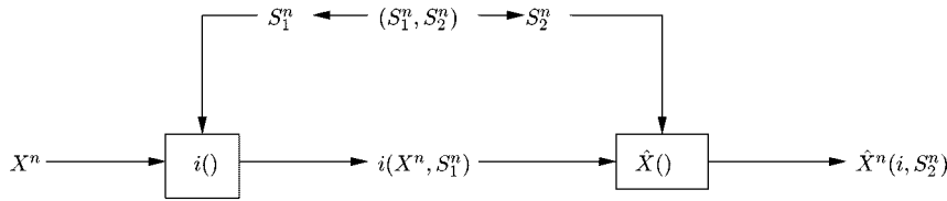
Fig. 4. Rate distortion with two-sided state information, where (X_i, S_{1,i}, S_{2,i}) are i.i.d. \sim p(x, s_1, s_2) : R(D) = \min_{p(u|x, s_1)p(\hat{x}|u, s_2)} [I(U; S_1, X) - I(U; S_2)] .
