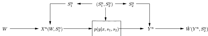
Fig. 3. Channel capacity with two-sided state information, where (S_{1,i}, S_{2,i}) are i.i.d. \sim p(s_1, s_2) : C = \max_{p(u,x|s_1)} [I(U; S_2, Y) - I(U; S_1)] .
