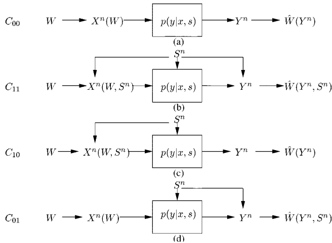
Fig. 1. Channels with state information. Four special cases. (a) C_{00} = \max_{p(x)} I(X; Y) . (b) C_{11} = \max_{p(x|s)} I(X; Y|S) . (c) C_{10} = \max_{p(u,x|s)} [I(U; Y) - I(U; S)] . (d) C_{01} = \max_{p(x)} I(X; Y|S) .
