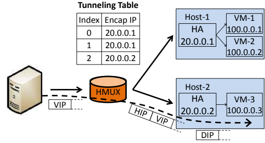
Figure 6: Load balancing in virtualized clusters.
