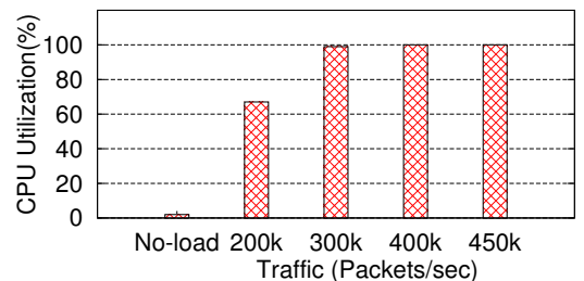
(b) CPU Utilization Figure 1: Performance of software Mux.
