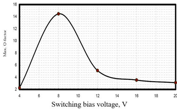
Figure 6. Variations of max. Q-factor against variations of switching bias voltage based LiNbO 3 Mach Zehnder Modulator at RF signal frequency of 100 GHz
