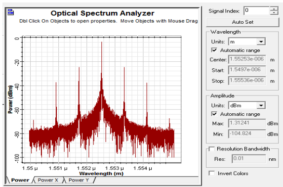
Figure 16. Max modulated power after LiNbO 3 MZM without predistortion technique at 40 Gb/s
