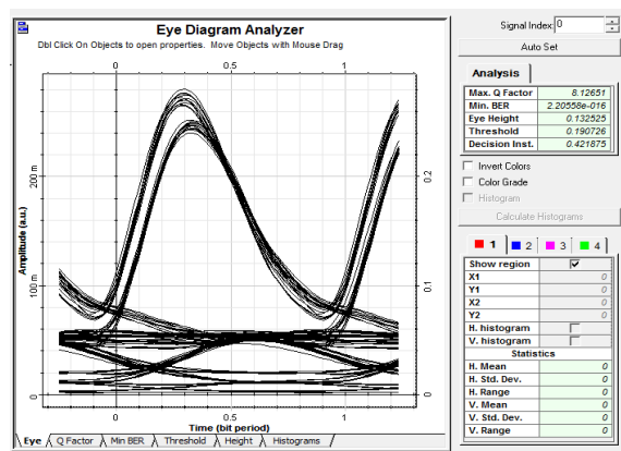
Figure 12. Eye diagram analyzer for NRZ/RZ (exponential rectangle shape) at 10 Gb/s
