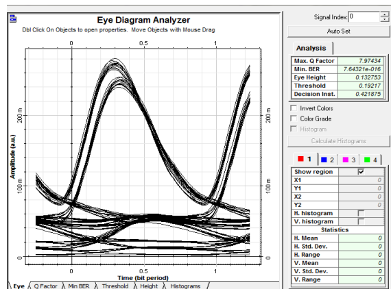
Figure 14. Eye diagram analyzer for NRZ/RZ (Gaussian rectangle shape) at 10 Gb/s
