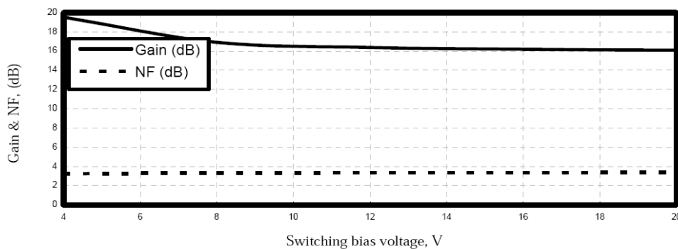
Figure 8. Gain, noise figure with switching bias voltage based LiNbO 3 Mach Zehnder Modulator at frequency of 100 GHz
