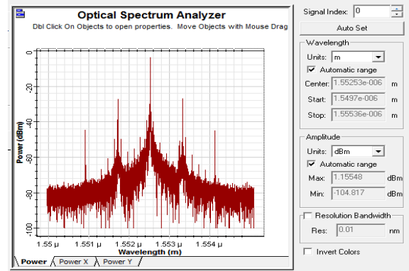
Figure 17. Maximum modulated power after LiNbO 3 Mach Zehender modulator in the presence of predistortion technique at 40 Gb/s
