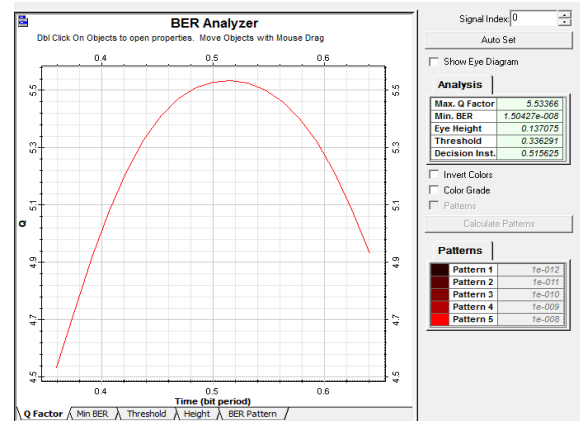
Figure 13. Bit error rate analyzer for NRZ/RZ (exponential rectangle shape) at 40 Gb/s
