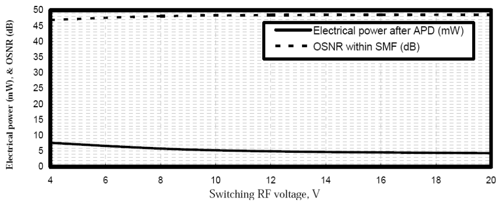
Figure 11. Electrical power and light signal/noise ratio versus switching RF voltage based LiNbO 3 Mach Zehnder Modulator at RF signal frequency of 100 GHz
