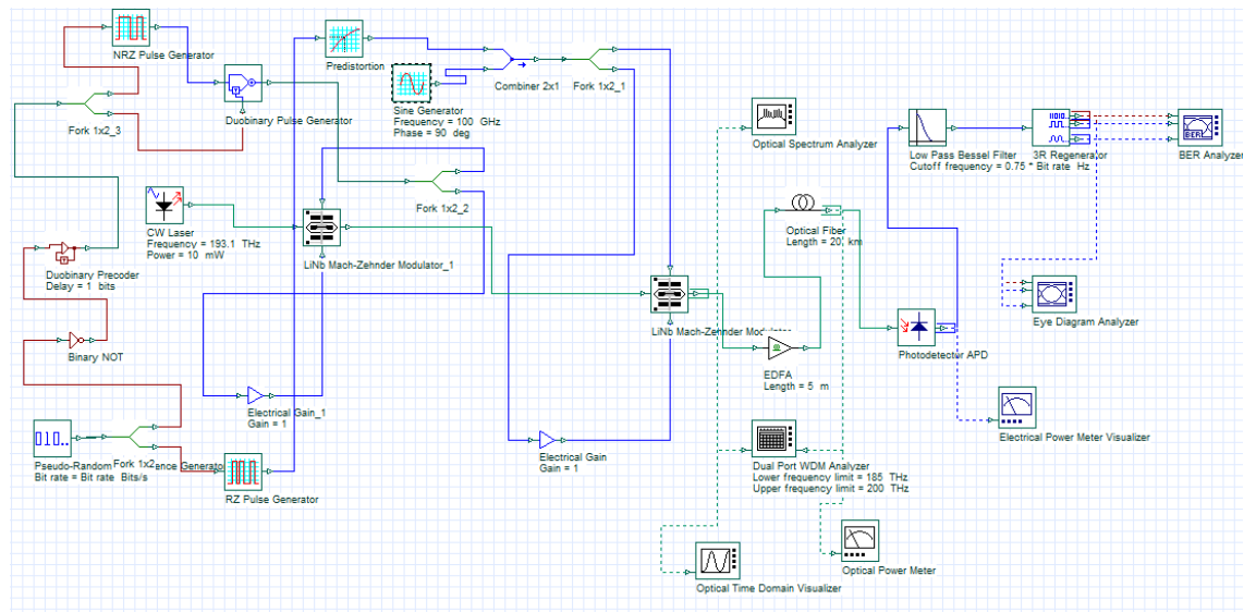
Figure 1. Schematic view of duobinary radio over fiber simulation modeling
