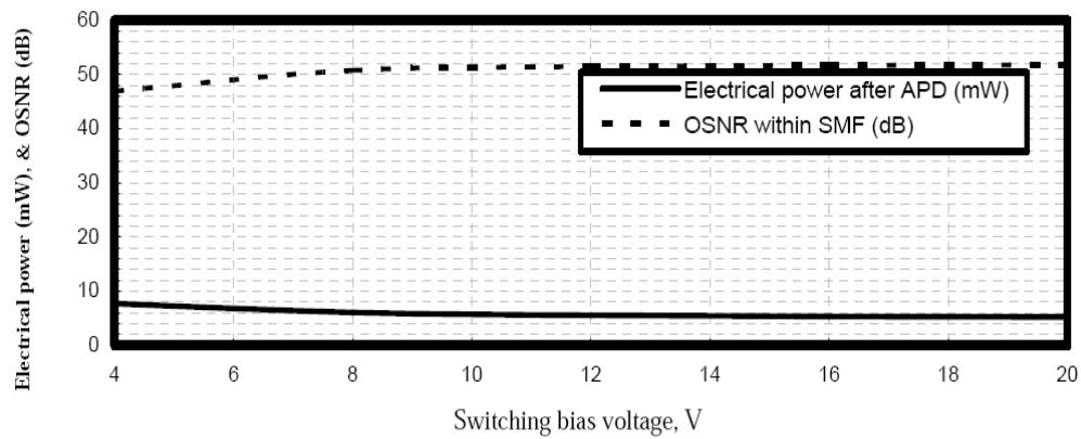
Figure 10. Variations of electrical power and light signal/noise ratio against variations of switching bias voltage based LiNbO 3 Mach Zehnder Modulator at RF signal frequency of 100 GHz
