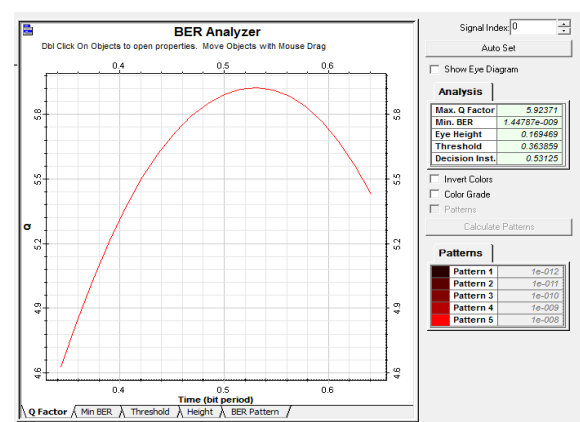
Figure 15. Eye diagram analyzer for NRZ/RZ (Gaussian rectangle shape) at 40 Gb/s
