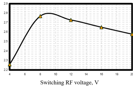
Figure 7. Max. Q-factor with switching voltage based LiNbO 3 Mach Zehnder Modulator at RF frequency of 100 GHz
