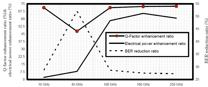
Figure 18. Q-factor enhancement ratio, electrical power enhancement ratio and BER reduction ratio in relation to RF signal frequency
