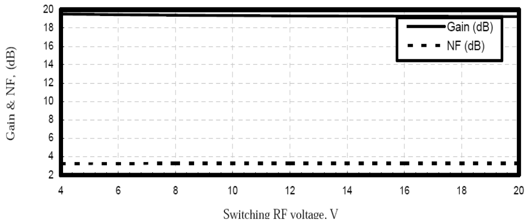
Figure 9. Gain, noise figure with switching RF voltage based LiNbO 3 Mach Zehnder Modulator at frequency of 100 GHz
