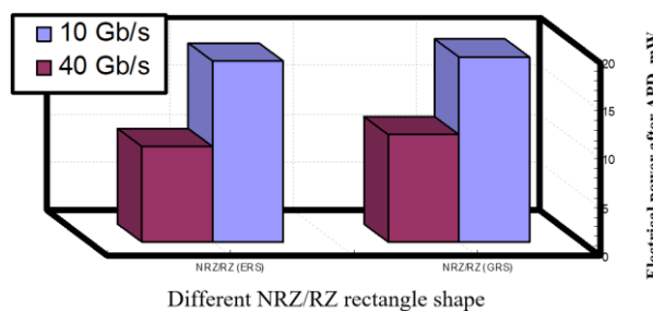
Figure 4. Electrical power after APD with overall system bit-rate based on different NRZ/RZ rectangle shape
