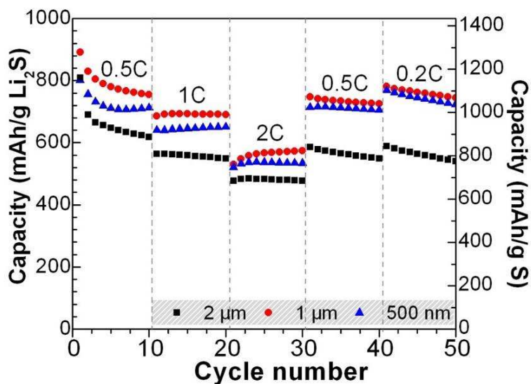
Figure S8. The rate performance of the 2 \mu\text{m} , 1 \mu\text{m} and 500 nm \text{Li}_2\text{S}@C particles.
