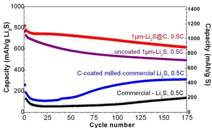
Figure S7. Cycling performance of the 1 \mu\text{m} \text{Li}_2\text{S}@C spheres (red) compared with uncoated 1 \mu\text{m} \text{Li}_2\text{S} spheres (purple), commercial \text{Li}_2\text{S} (black) and carbon-coated milled-commercial \text{Li}_2\text{S} (blue) at 0.5C rates. (Electrode composition: \text{Li}_2\text{S}:\text{C}:\text{PVP}=60:35:5 by weight; 1.0-1.5 \text{mg Li}_2\text{S}/\text{cm}^2 )
