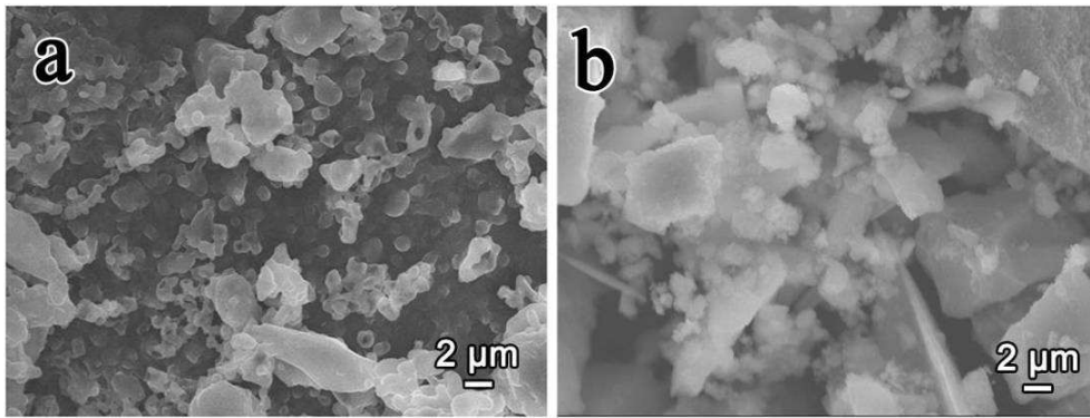
Figure S3. (a) Synthesis of Li 2 S with toluene, but no heat treatment; (b) Synthesis of Li 2 S without toluene. (The other synthesis processes are the same as described in experimental section)
