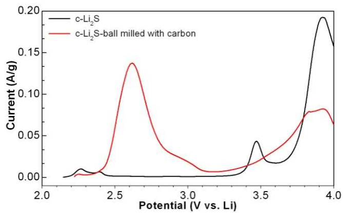
Figure S10. CVs of the commercial \text{Li}_2\text{S} (c- \text{Li}_2\text{S} ) materials before and after ball-milling at a scan rate of 0.025 mV/s. (Electrode composition: \text{Li}_2\text{S} : C: PVP= 60: 35: 5 by weight; 1.0-1.5 mg \text{Li}_2\text{S}/\text{cm}^2 )
