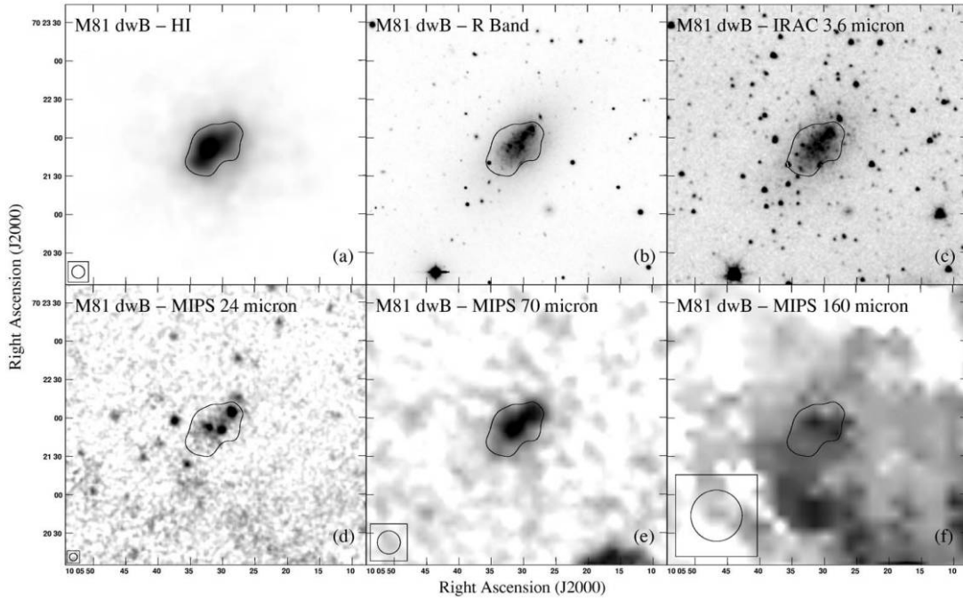
FIG. 6.—M81 dwB: (a) integrated THINGS H I map (contour shown at N_{\text{H I}} = 10^{21} \text{ cm}^{-2} in all panels); (b) R -band image; (c) IRAC 3.6 \mu\text{m} image; (d, e, and f) 24, 70, and 160 \mu\text{m} images, respectively. The sizes of the H I and MIPS beams are given in the lower left corners of their respective panels.
