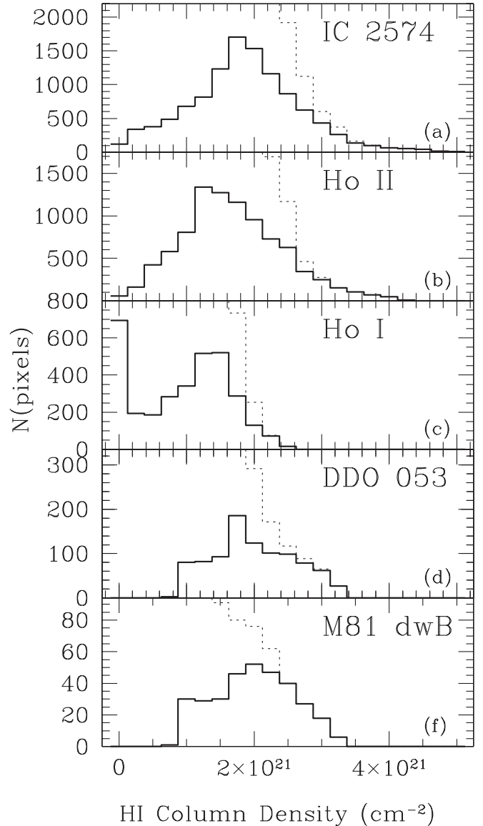
FIG. 9.— Solid histogram : Distribution of the 70 \mu\text{m} flux density above a threshold of 1.8 \text{ MJy sr}^{-1} ( \sim 5\sigma ) as a function of H I column density. Dashed histogram : Total distribution of H I column densities.
