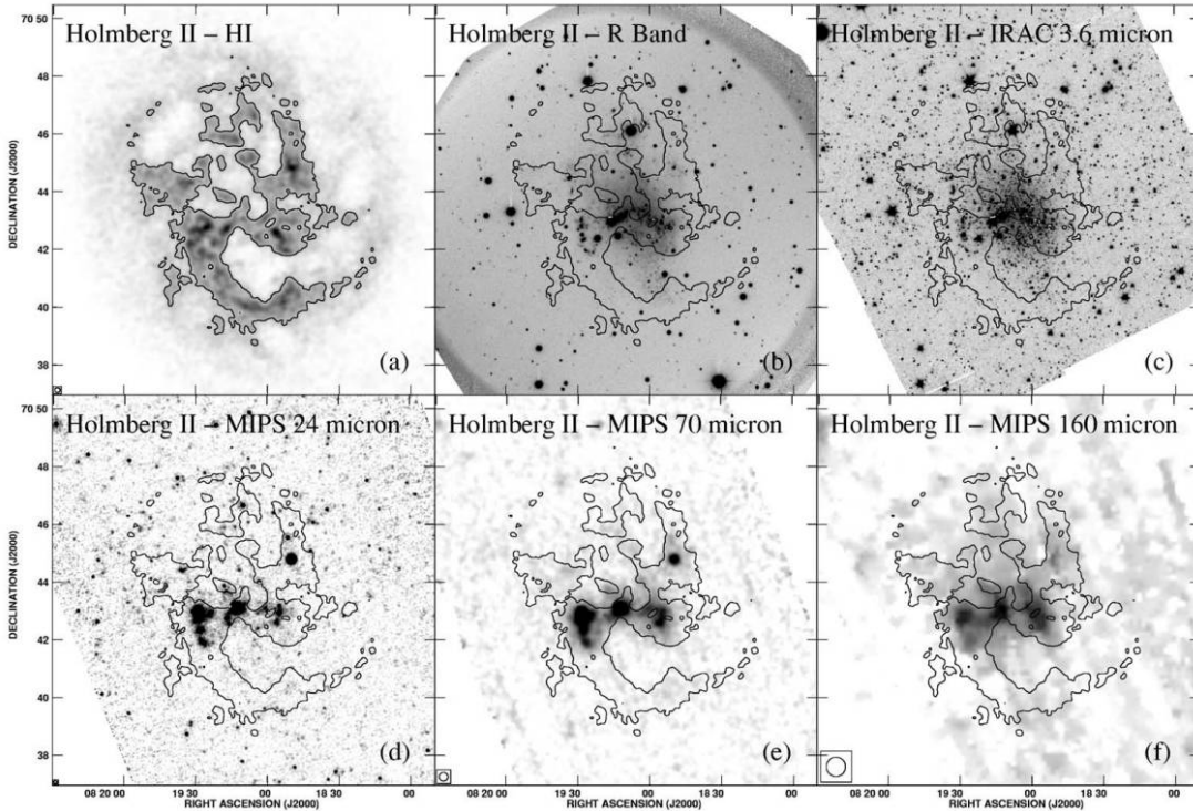
FIG. 2.—Holmberg II: (a) integrated THINGS H I map (contour shown at N_{\text{H I}} = 10^{21} \text{ cm}^{-2} in all panels); (b) R -band image; (c) 3.6 \mu\text{m} image; (d, e, and f) 24 , 70 , and 160 \mu\text{m} images, respectively. The sizes of the H I and MIPS beams are given in the lower left corners of their respective panels.
