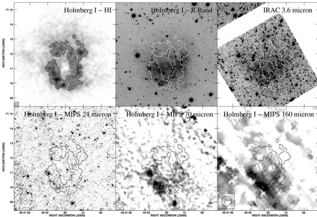
FIG. 3.—Holmberg I: (a) integrated THINGS H I map (contour shown at N_{\text{H I}} = 10^{21} \text{ cm}^{-2} in all panels); (b) R -band image; (c) IRAC 3.6 \mu\text{m} image; (d, e, and f) 24 , 70 , and 160 \mu\text{m} images, respectively. The sizes of the H I and MIPS beams are given in the lower left corners of their respective panels.
