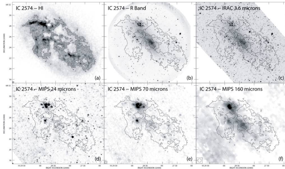
FIG. 1.—IC 2574: (a) integrated THINGS H I map (contour shown at N_{\text{HI}} = 10^{21} \text{ cm}^{-2} in all panels); (b) R -band image; (c) IRAC 3.6 \mu\text{m} image; (d, e, and f) 24, 70, and 160 \mu\text{m} images, respectively. The sizes of the H I and MIPS beams are given in the lower left corners of their respective panels.
