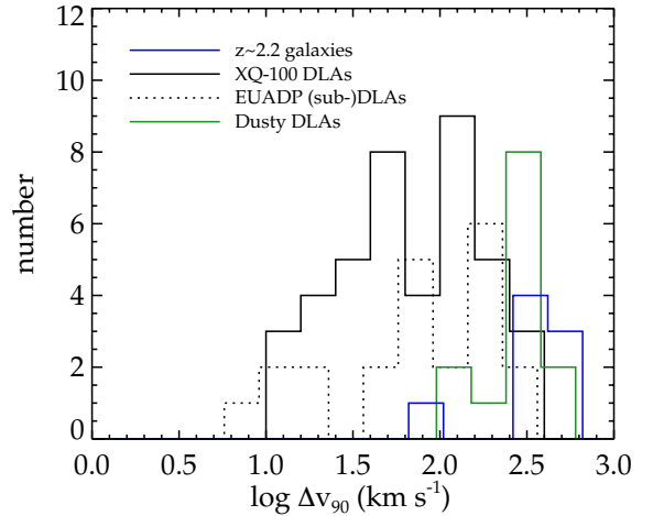
FIG. 11.— Velocity width distributions of the ESI galaxy sample compared to DLA absorption systems in quasar spectra. We show histograms of low ion \Delta V_{90} from the XQ-100 survey (Berg et al. 2016), EUADP sample (Quiret et al. 2016), and dusty DLAs selected on the basis of 2175 Å dust attenuation features (Ma et al. 2017). Galaxies in our sample have broader velocity distributions than typical DLAs, lying at or beyond the extreme tail of the XQ-100 and EUADP samples. The dusty DLAs have comparable velocity widths. We estimate \Delta V_{90} = 3.29\sigma_v for the galaxy sample, noting that redshifted outflowing gas on the far side of the galaxies would further increase \Delta V_{90} by up to 0.3 dex, exacerbating the discrepancy with typical DLAs.
