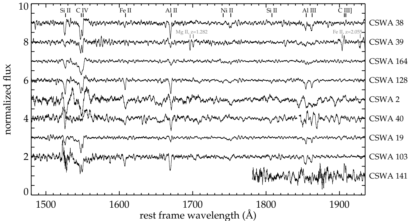
FIG. 1.— Spectra of the nine galaxies in the ESI sample in the rest-frame wavelength range 1500–1900 Å, normalized and offset for clarity, ordered from highest (top) to lowest redshift. In the case of CSWA 141 we show only the spectrum redward of 4300 Å in the observed frame. The spectra are smoothed to \sim 250 \text{ km s}^{-1} FWHM resolution for display purposes. Several prominent features are labeled at top. We also label strong lines from two intervening absorption systems identified in the spectrum of CSWA 39. Significant dispersion can be seen in the equivalent width of features such as Si II \lambda 1526 and Al II \lambda 1670 , which are typically optically thick and therefore trace the covering fraction and velocity profile of low-ionization gas. Weaker lines such as Si II \lambda 1808 and Ni II \lambda 1741, \lambda 1751 are additionally sensitive to the gas column density.
