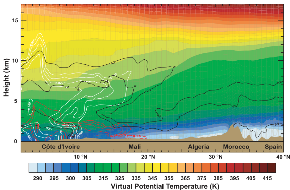
Fig 11. Results from the regional model COSMO–MUSCAT. Meridional-vertical cross-section along 5°W at 1200 UTC on 17 January 2008 showing virtual potential temperature (K, colours), specific humidity ( \text{g kg}^{-1} , black), and extinction coefficients at 550 nm ( \text{km}^{-1} ) due to dust (red) and biomass-burning aerosol (white).
