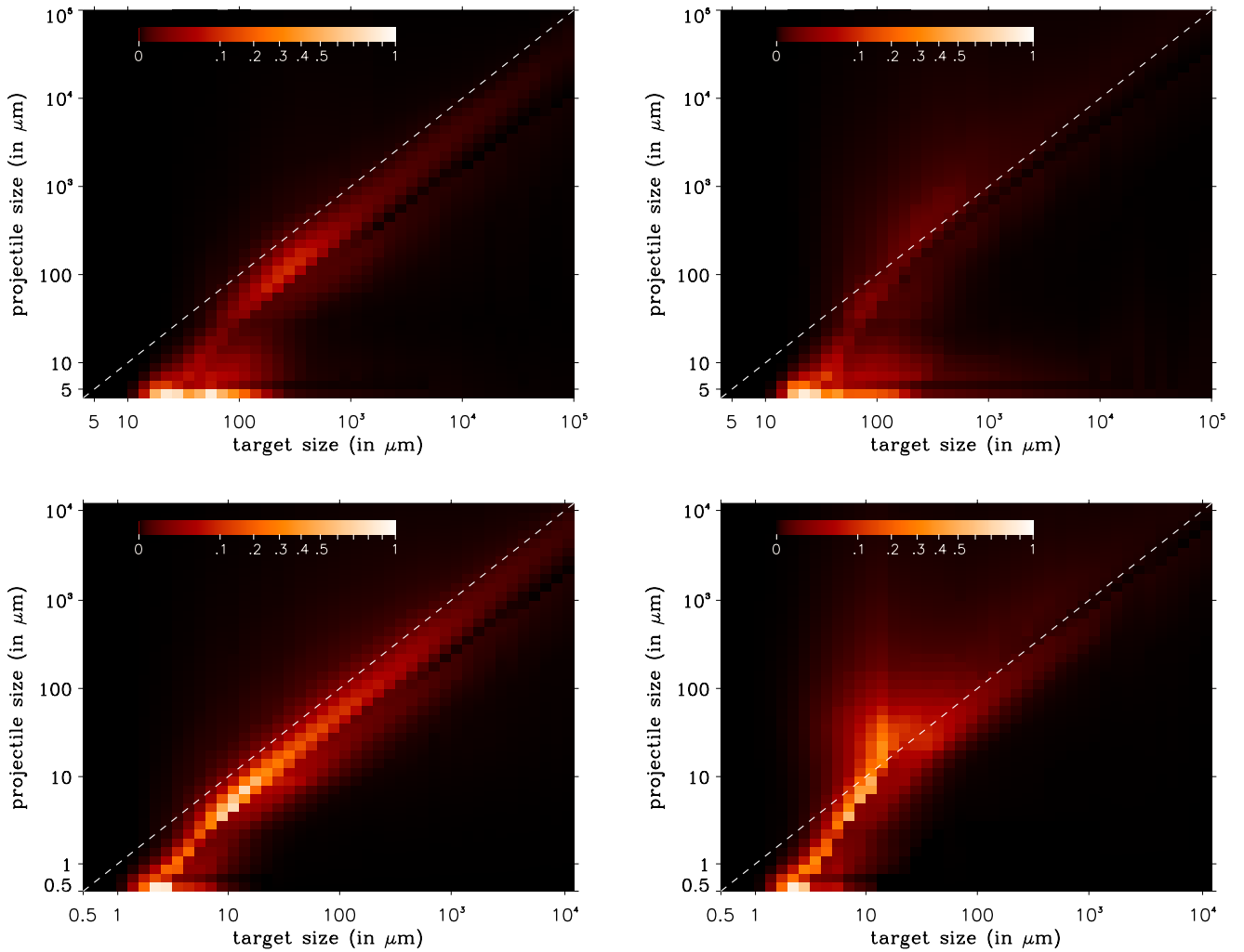
Fig. 2. Disc-integrated and normalized production rates of s \leq 10 \mu\text{m} dust as a function of target and projectile sizes. These maps are estimated, at collisional steady-state, for the “control runs” where the s_{\text{surf}} criteria is turned off. This allows for an easy comparison with Fig. 1 by directly showing which high s_{\text{surf}}(i, j) regions will have a significant damping effect on the small-dust production rate. Upper left panel: A-star primary and \langle e \rangle = 0.075 . Upper right: A-star primary and \langle e \rangle = 0.01 . Bottom left: solar-type primary and \langle e \rangle = 0.075 . Bottom right: solar-type primary and \langle e \rangle = 0.01 .
