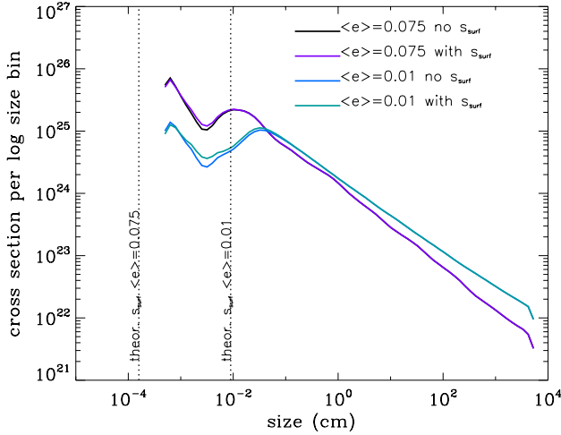
Fig. 3. A-star case. Geometrical cross-section as a function of particle size, at t = 10^7 yr, integrated over the whole 50–100 au disc, for both the dynamically “hot” ( \langle e \rangle = 0.075 ) and “cold” ( \langle e \rangle = 0.01 ) cases. For each case, a reference run with the s_{\text{surf}} constraint switched-off is also presented. The two vertical dotted lines represent the analytical values given by Eq. (2).
