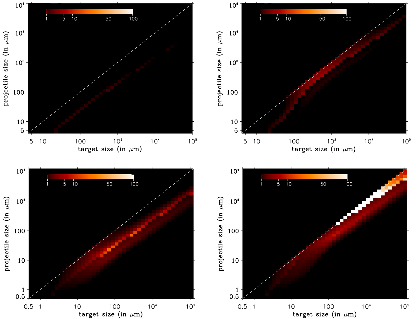
Fig. 1. Disc-integrated mean values of the s_{\text{surf}}/s_{\text{blow}} ratio for all possible target-projectile pairs of sizes s_i and s_j . Upper left panel: A-star primary and \langle e \rangle = 0.075 . Upper right: A-star primary and \langle e \rangle = 0.01 . Bottom left: solar-type primary and \langle e \rangle = 0.075 . Bottom right: solar-type primary and \langle e \rangle = 0.01 . The dashed white line delineates the s_i = s_j diagonal of equal-sized impactors.
