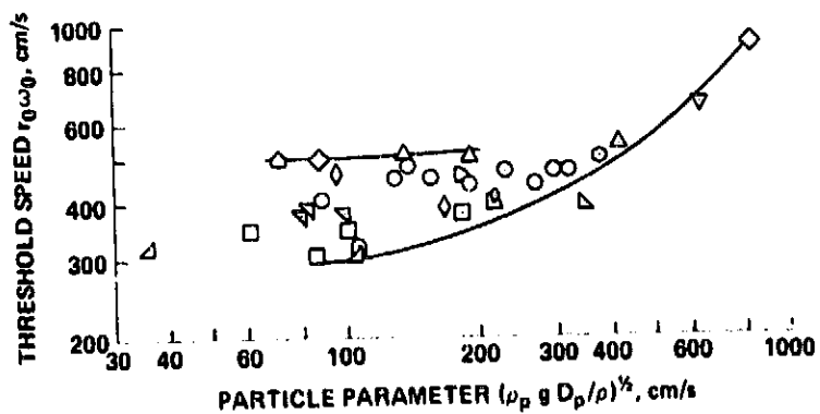
Figure 22. - Characteristic vortex threshold speed r_0 \omega_0 = (\Delta p / \rho)^{1/2} as a function of particle parameter. Note that for large particles the pressure difference \Delta p is nearly equal to the weight per unit area of a single layer of particles. For small particles the pressure difference \Delta p ranges up to nearly ten times the weight per unit area of a single layer. One explanation for the difference is small particle cohesion (interparticle stress \sigma_f ).
