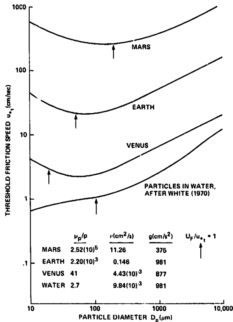
Figure 9.- Comparison of threshold friction speed vs particle diameter for Earth, Mars, Venus, and in liquid. In all cases except liquid, there is an "upturn" in the speed needed to set smaller grains in motion; thus, on each planet, there is an optimum particle size for movement by lowest winds (ref. 36).
