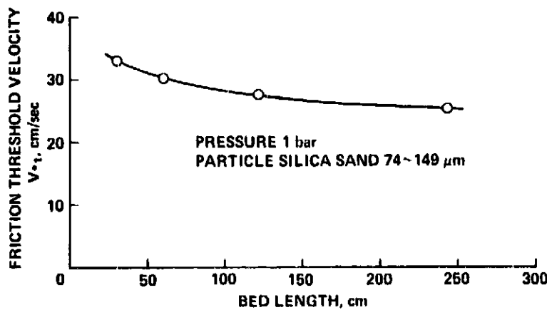
Figure 13.- Effect of length of particle test bed on threshold at 1 bar pressure for 74-149 \mu m silica sand. Lengths shorter than about 1.5 m result in anomalously high friction threshold.
