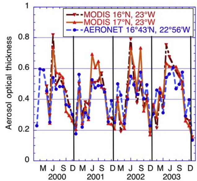
Figure 17. Monthly averages of the aerosol optical thickness measured by AERONET in Capo Verde and derived from MODIS around the location of the Sun photometer over the ocean. For the 3 full years of operation the MODIS optical thickness was 0.40–0.42, and AERONET was 0.39–0.43. The MODIS data are from Terra at \sim 1030 LT, and the AERONET data are averaged on the daily hours. The AERONET level 1.0 data are used with only partial cloud screening due to possible screening of heavy dust with the accompanied clouds. Both data sets show similar seasonal cycle of the aerosol with maximum in the June–September time frame.
