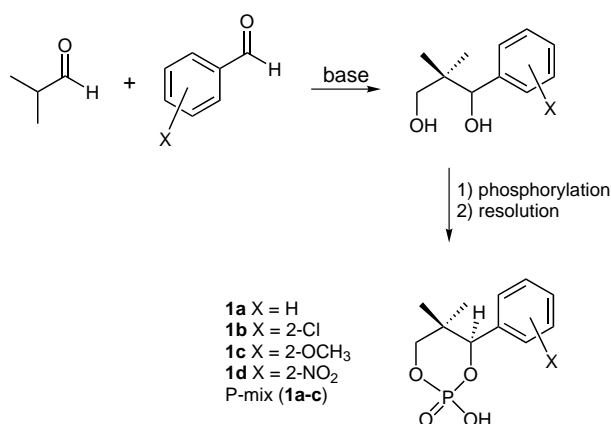
Scheme 1 Synthesis of cyclic phosphoric acids
