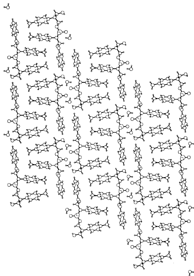
Figure 5 Stacking plot of 18a+18b/19 with 18a:18b , 17:83
