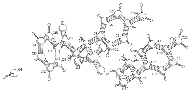
Figure 4 Crystal structure of 18a+18b/19 with 18a:18b , 17:83
