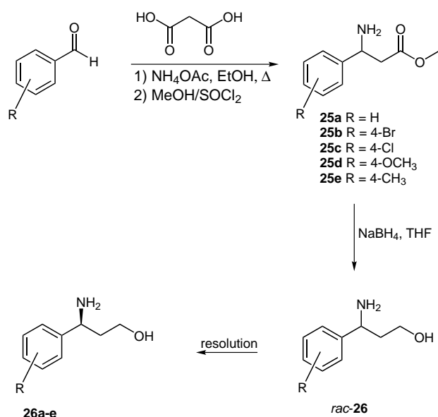
Scheme 6 Synthesis of amino esters 25 and amino alcohols 26
