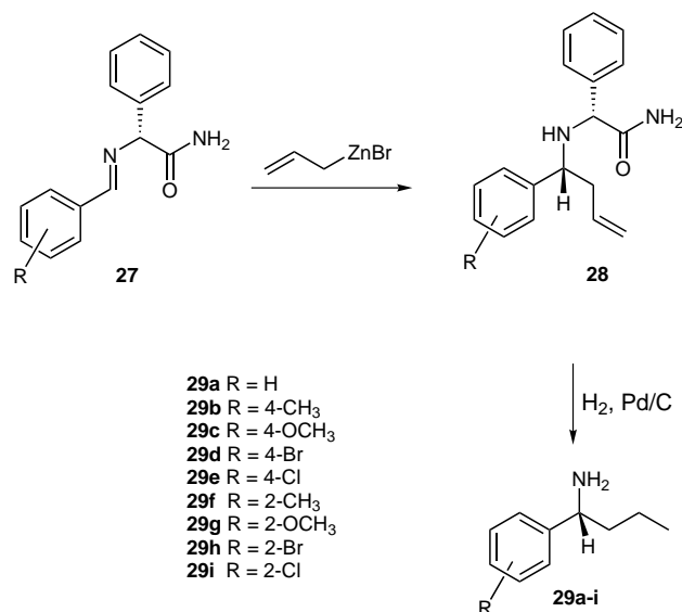
Scheme 7 Diastereoselective allylzinc additions to imines of ( R )-phenylglycinamide 27
