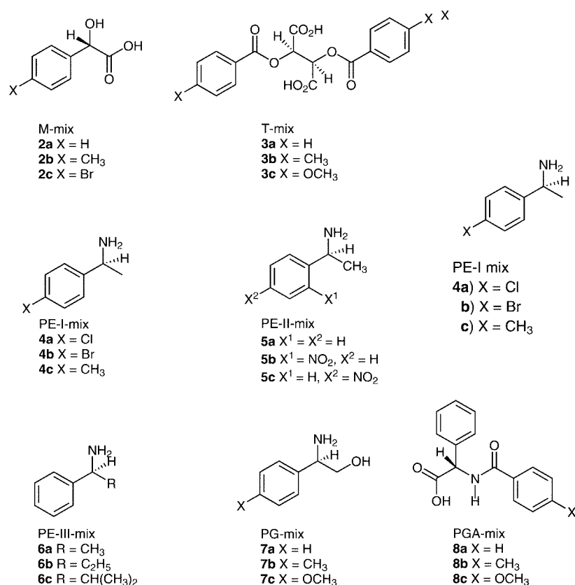
Figure 1 Families of resolving agents
