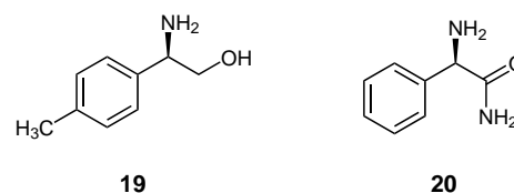
Figure 3 ( R )-4-methylphenylglycinol 19 and D-phenylglycinamide 20
