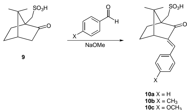
Scheme 2 Condensation of benzaldehydes with camphor sulfonic acid 9
