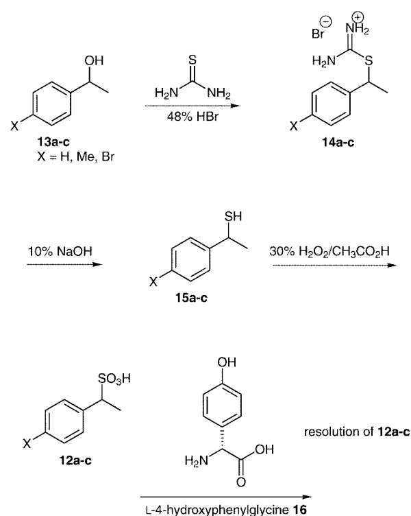
Scheme 3 Synthesis of 1-phenylethanesulfonic acid 12
