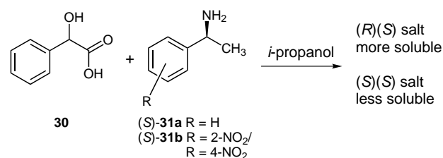
Scheme 8 Resolution of 30 with 31a in the presence of 31b
