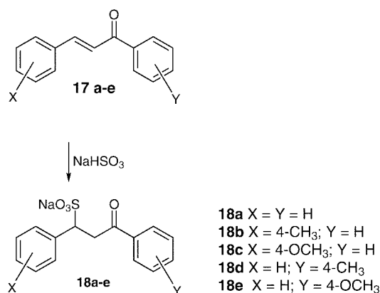
Scheme 4 Addition of sodium bisulfite to chalcones 17a–e
