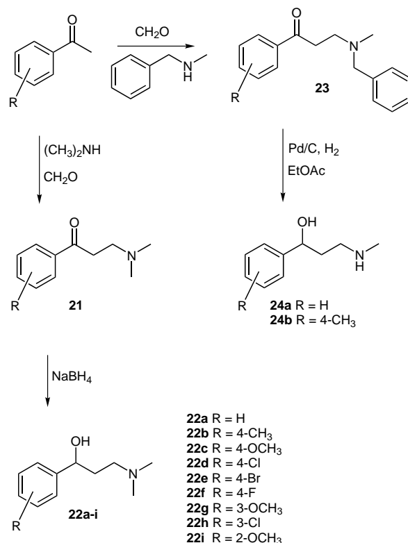
Scheme 5 Mannich approach to amino alcohols 22 and 24
