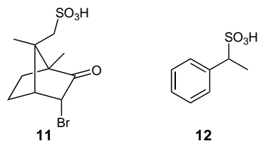
Figure 2 Bromo camphor sulfonic acid 11 and 1-phenylethanesulfonic acid 12
