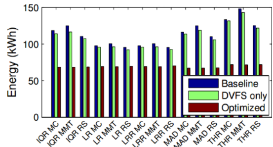
Fig. 2: Average energy consumption comparison per test
