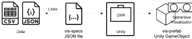
Fig. 3. DXR overview: A vis-specs file references the data file and holds the design declaration. It gets interpreted by DXR to generate a visualization that is represented as a vis-prefab GameObject in Unity.
