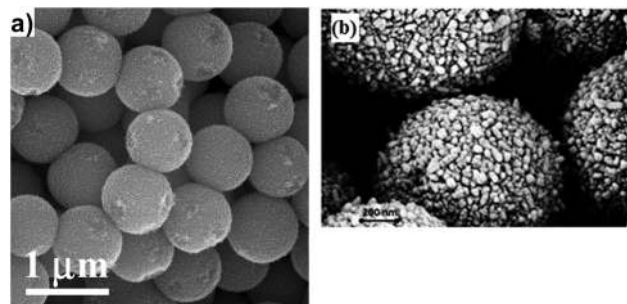
Fig. 17 SEM micrographs of mesoporous \text{TiO}_2 microbeads. (a) Adapted with permission from ref. 223. Copyright 2010 American Chemical Society. (b) Adapted from ref. 222 with permission from The Royal Society of Chemistry, copyright 2014.
