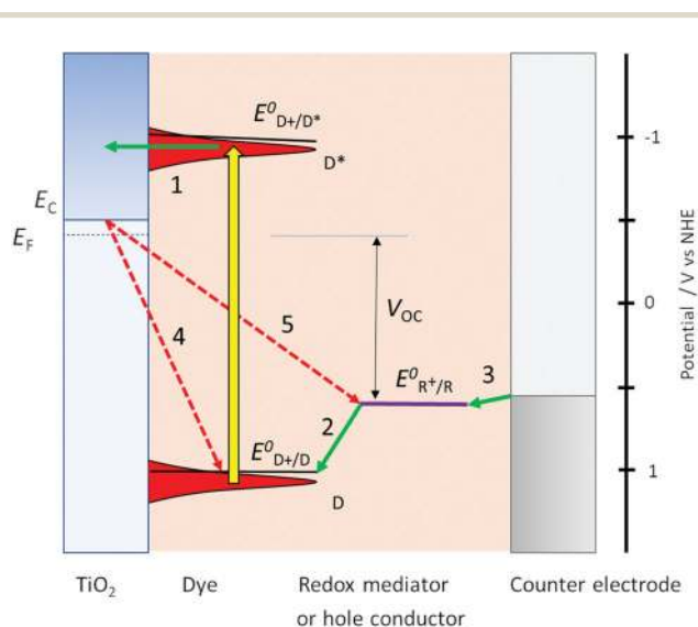
Fig. 3 Basic diagram of the dye-sensitized solar cell, displaying working mechanism and energy levels.
