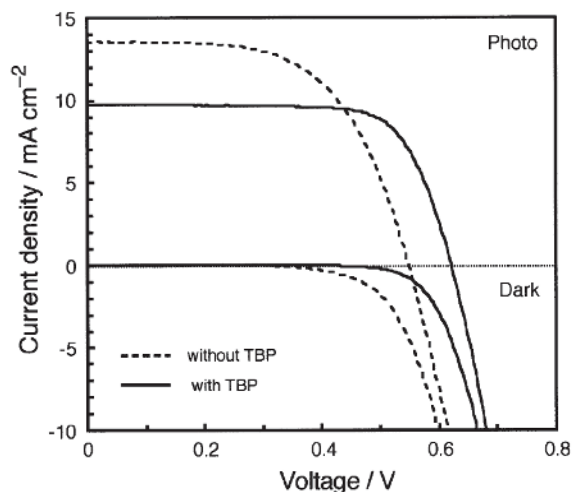
Fig. 19. Current–voltage curves obtained for NKX-2311-sensitized TiO 2 solar cells in an electrolyte of 0.6M DMPIII–0.1M LiI–0.05M I2 in methoxyacetonitrile: (– –) without TBP, (–) with 0.5M TBP (From Hara et al., 2003).
