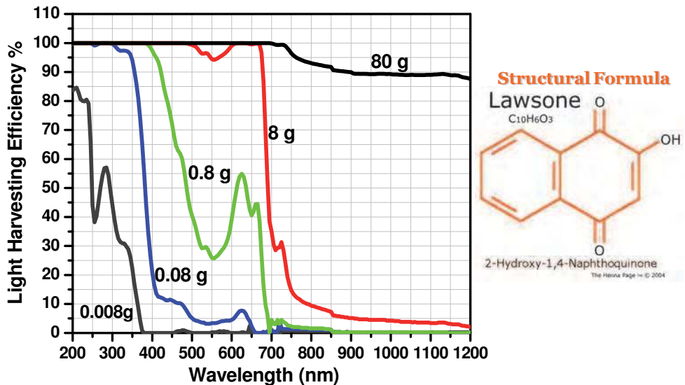
Fig. 10. Light harvesting efficiency of Henna extract at different concentrations. Data are given in grams of Henna powder per 100 ml of methanol as solvent. Also, shown the structural formula of Lawsone molecule that is responsible for the characteristic color of Henna (From www.hennapage.com ).
