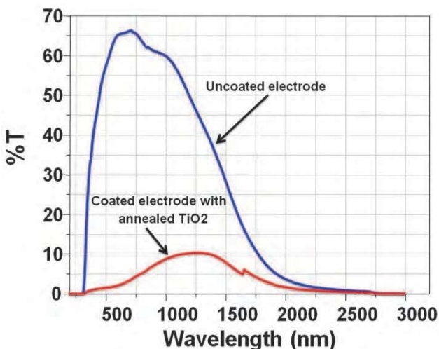
Fig. 3. Transmittance of conductive glass electrode before and after being coated with nanostructured TiO_2 layer.
