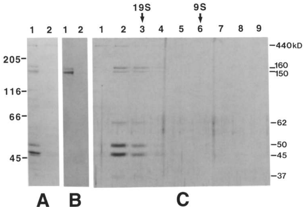
Figure 2. An activator of vesicle motility is a complex of proteins, a prominent component of which is a \sim 150 -kD doublet. (A and B) Immunodepletion of the 150-kD monoQ fraction with Sepharose-bound mAb 150.1. (A) Coomassie blue-stained gel and (B) corresponding immunoblot with mAb 150.1 of the 150-kD monoQ fraction after incubation with a control, nonspecific antibody (lane 1) and after immunodepletion with mAb 150.1 (lane 2). Positions of molecular weight markers (in kilodaltons) are marked at the left of A. (C) Cosedimentation of the proteins eluting with the 150-kD polypeptides from the monoQ column. The material shown in Fig. 1 A, lane 3, was sedimented into a 5–20% sucrose gradient and fractions analyzed by gel electrophoresis. Positions of purified proteins (thyroglobulin [19S] and amylase [9S]) sedimented in a parallel gradient are noted by arrows.
