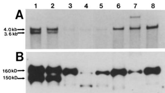
Figure 6. Three mRNAs encode at least three dynactin isoforms in various chicken tissues. (A) RNA blot analysis of total RNA isolated from various chicken tissues probed with the cloned dynactin cDNA from p150A. (B) Immunoblot analysis of dynactin isoforms in chicken tissue extracts probed with mAb 150.1. Lane 1, 11-d embryonic chick brain; lane 2, adult brain; lane 3, cardiac muscle; lane 4, liver; lane 5, kidney; lane 6, smooth muscle; lane 7, skeletal muscle; lane 8, MSB cells, a Marek's virus transformed lymphoblastoid line. Sizes are shown at the left in kilobases or kilodaltons, respectively, for A and B.
