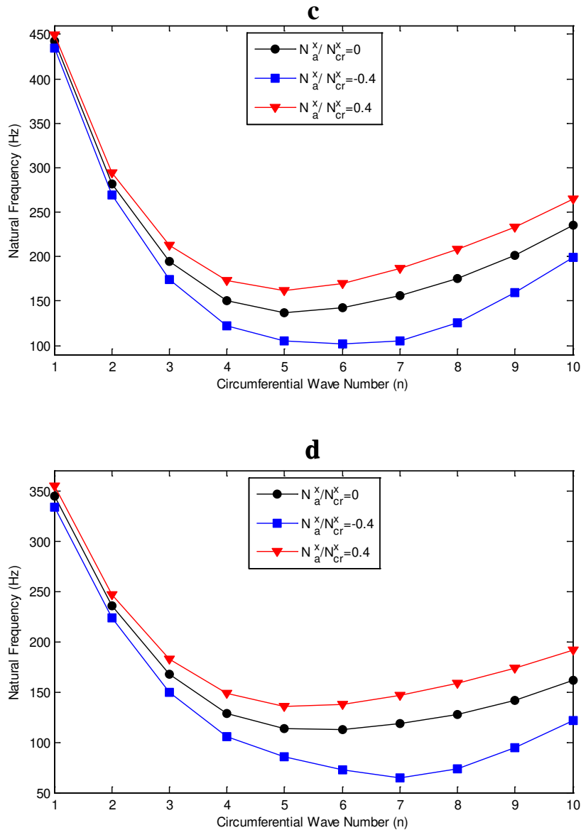
Figure 13 Variation of natural frequencies for the non-rotating stiffened composite conical shell with circumferential wave number at various cone angles, (a) \alpha=0^\circ , (b) \alpha=15^\circ , (c) \alpha=30^\circ , (d) \alpha=45^\circ . ( L=1m , a=0.25m , h=3mm , m=1 , N_s=N_r=5 , [0^\circ/90^\circ/0^\circ] , Cs-Cl)
