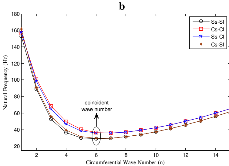
Figure 7 Variation of natural frequencies for the composite conical shell having circumferential wave number for different boundary conditions, (a) unstiffened shell, (b) stiffened shell N_s=N_r=10 . ( L=3m , a=0.5m , h=3mm , \alpha=30^\circ , m=1 , \Omega=0 , [0^\circ/90^\circ/0^\circ] )
