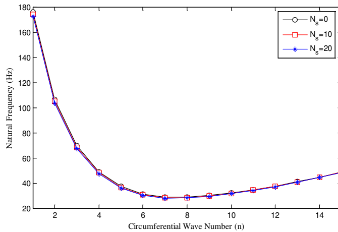
Figure 9 Variation of natural frequencies for the composite conical shell with circumferential wave number in various numbers of stringers ( L=3m, a=0.5m, h=3mm, \alpha=20^\circ, m=1, \Omega=0, [0^\circ/90^\circ/0^\circ], Cs-CI )
