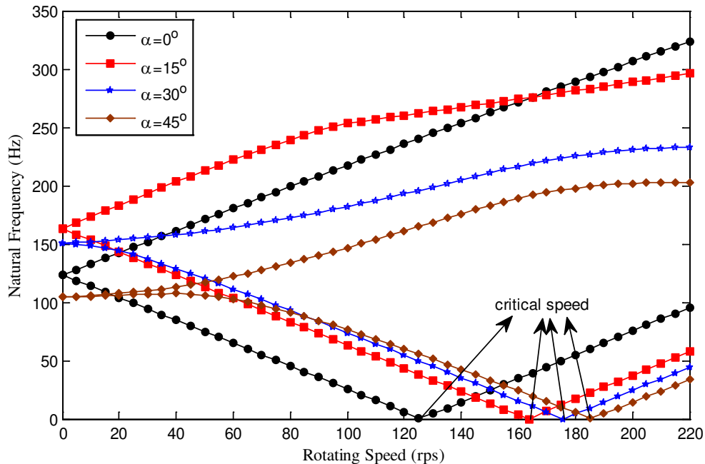
Figure 11 Variation of natural frequency of the rotating stiffened laminated conical shell with rotating speed at various cone angles ( L=3\text{m} , a=0.5\text{m} , h=3\text{mm} , m=n=1 , N_s=N_r=10 , [0^\circ/90^\circ/0^\circ] , Ss-Sl)
