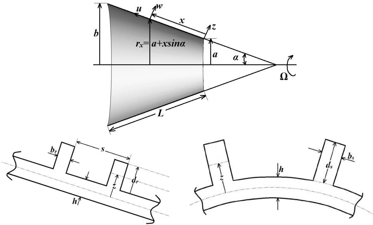
Figure 1 Geometry of stiffened rotating conical shell structure
