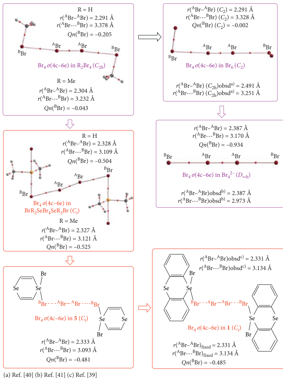
FIGURE 3: Sequence in the stabilization of \text{Br}_4 \sigma(4c-6e) , starting from those in G(A) to 1 via those of G(B).
