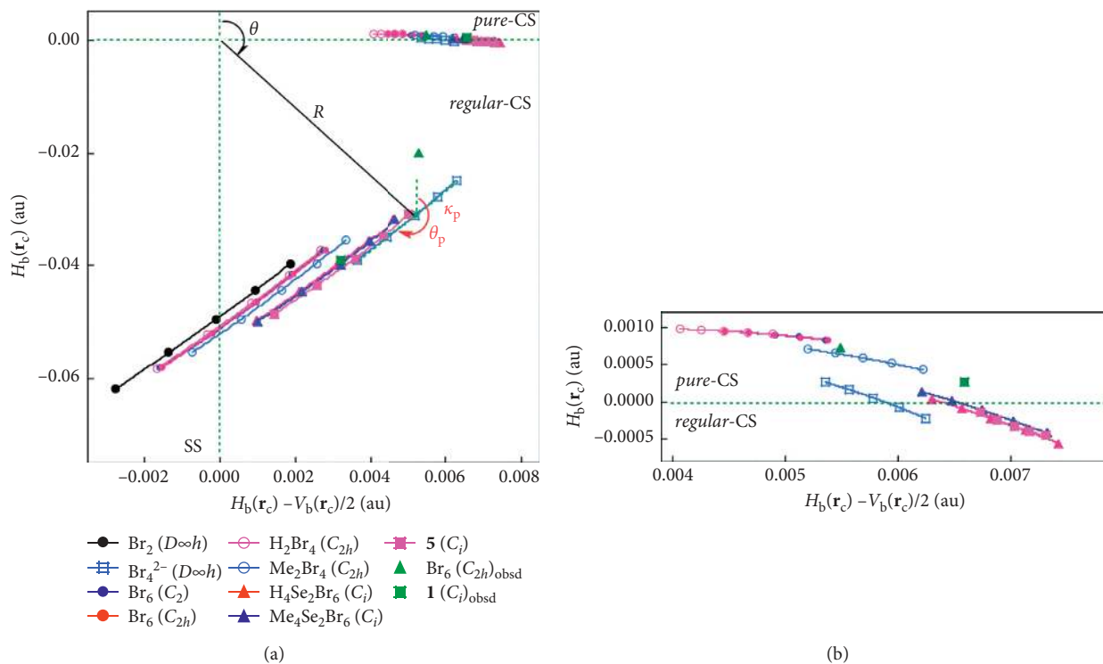
FIGURE 4: QTAIM-DFA plots of H_b(\mathbf{r}_c) versus H_b(\mathbf{r}_c) - V_b(\mathbf{r}_c)/2 for {}^A\text{Br}-*-\text{}^A\text{Br} (a) and {}^A\text{Br}-*-\text{}^B\text{Br} (b) in \text{Br}_4 \sigma(4c-6e) of the species in Table 1, together with those of the perturbed structures generated with CIV. Marks and colours for the species are shown in the figure.
