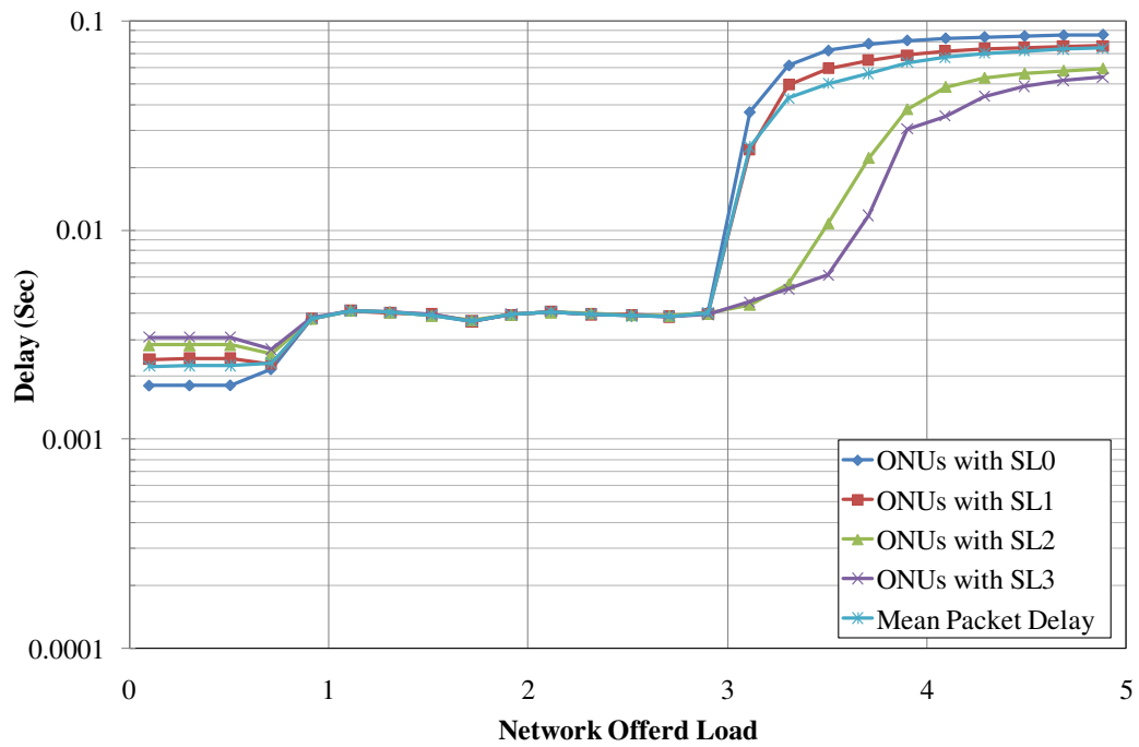
Figure 6-9: Packet delay performance for EBDMW-GPON for different service levels
