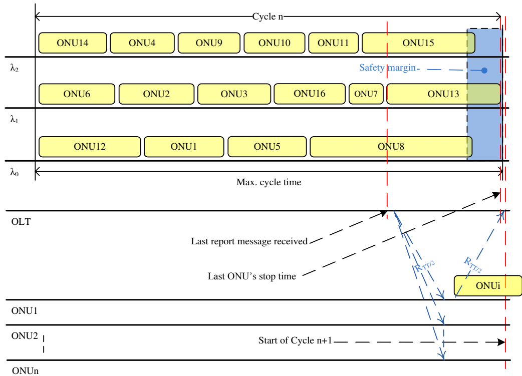
Figure 6-1: ONU traffic allocation in view of the ADMW algorithm
