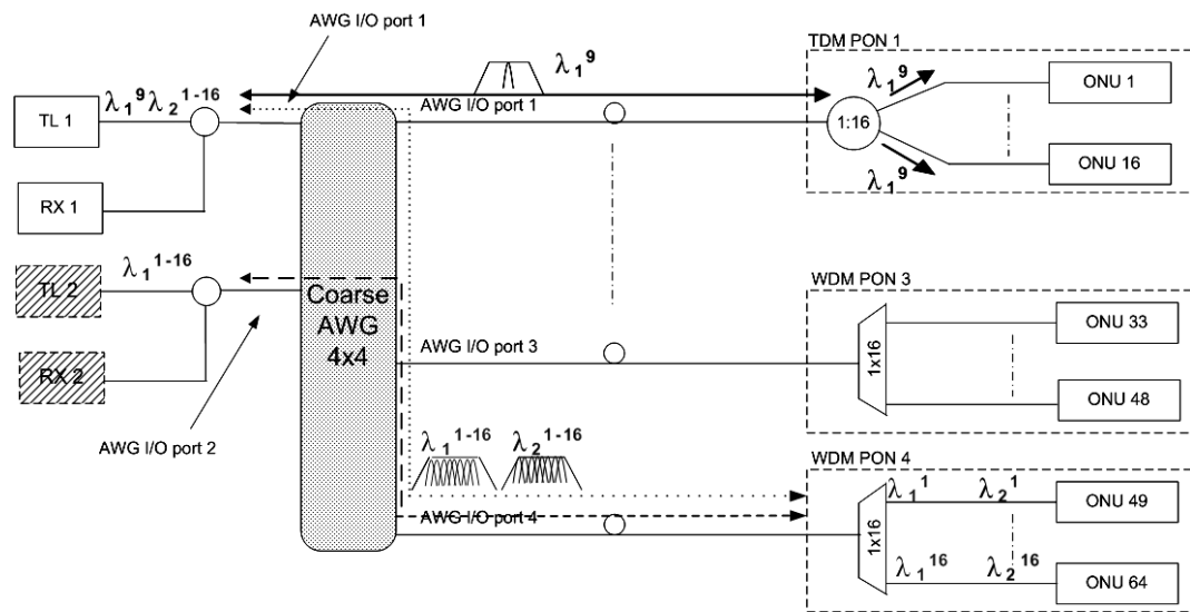
Figure 3-2: Multi-PON architecture [50]
