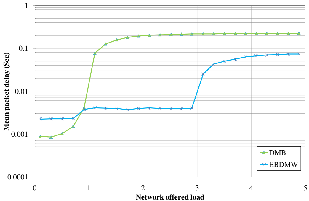
Figure 6-13: Mean packet delay performance for DMB and EBDMW GPON
