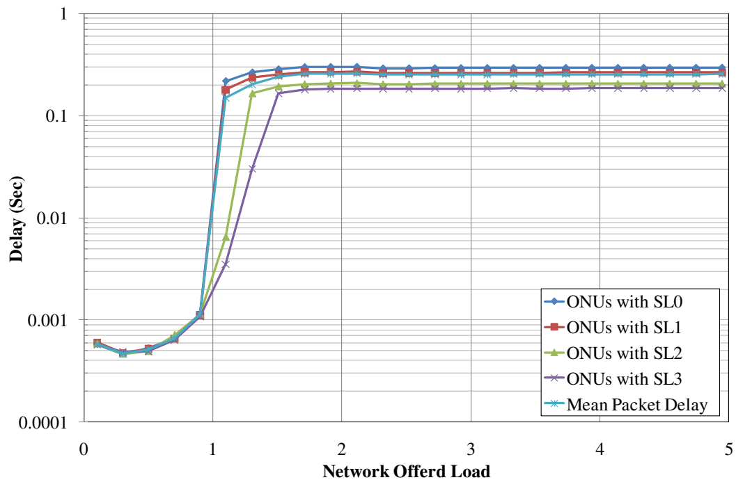
Figure 4-14: Simulated packet delay performance with four SLA DMB-GPON
