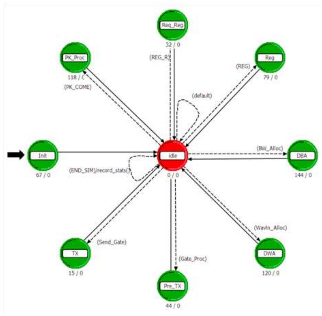
Figure 4-4: OLT process Model
