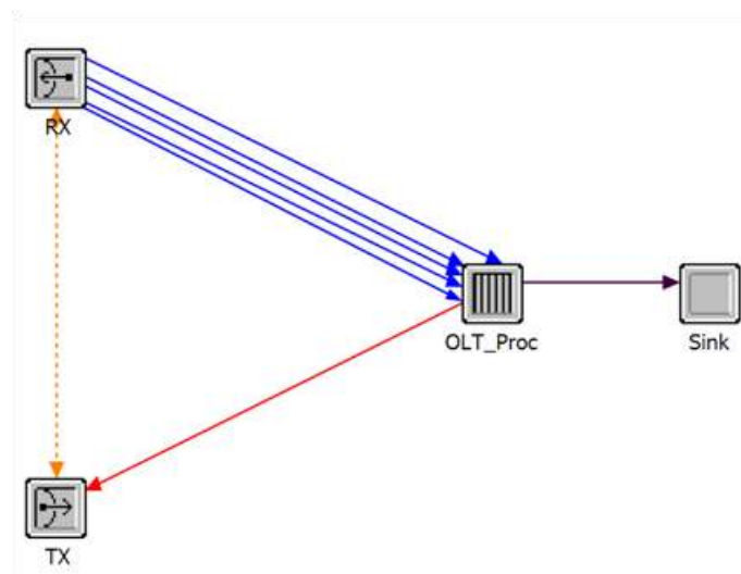
Figure 4-3: OLT node Model
