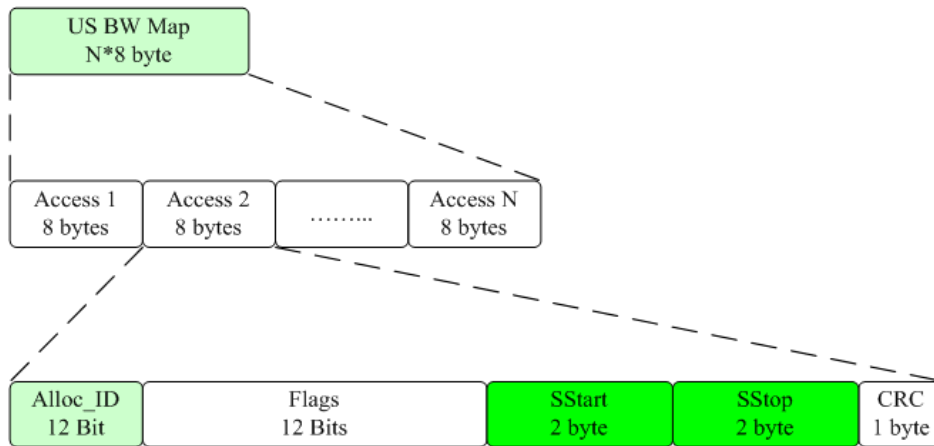
Figure 3-6: ITU-T G 984.3 PCBd US BW Map [8]
