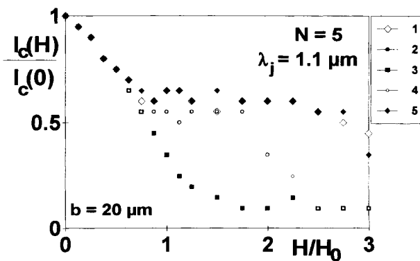
FIG. 17. Simulation of I_c(H) of the five Josephson junctions, labeled 1–5, in a stack of N=5 . For the simulation typical BSCCO parameters have been used.
