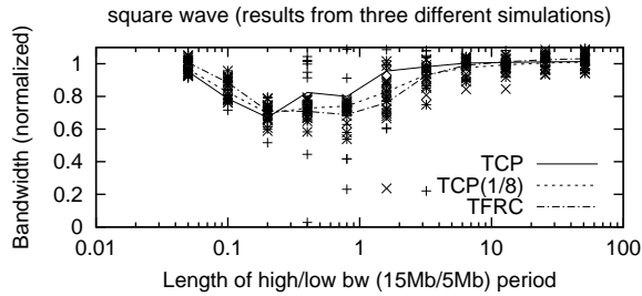
Figure 14: Effect of varying bandwidth on link utilization.
