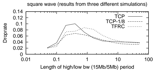
Figure 15: The corresponding packet loss rate.
