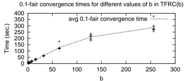
Figure 12: Time (in seconds) for convergence to 0.1-fairness for TFRC(b) flows.
