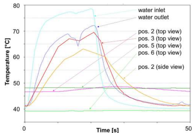
Fig. 15 Temperature profiles at measuring points with variothermal tempering (40/80 °C) of the ejector mold insert
