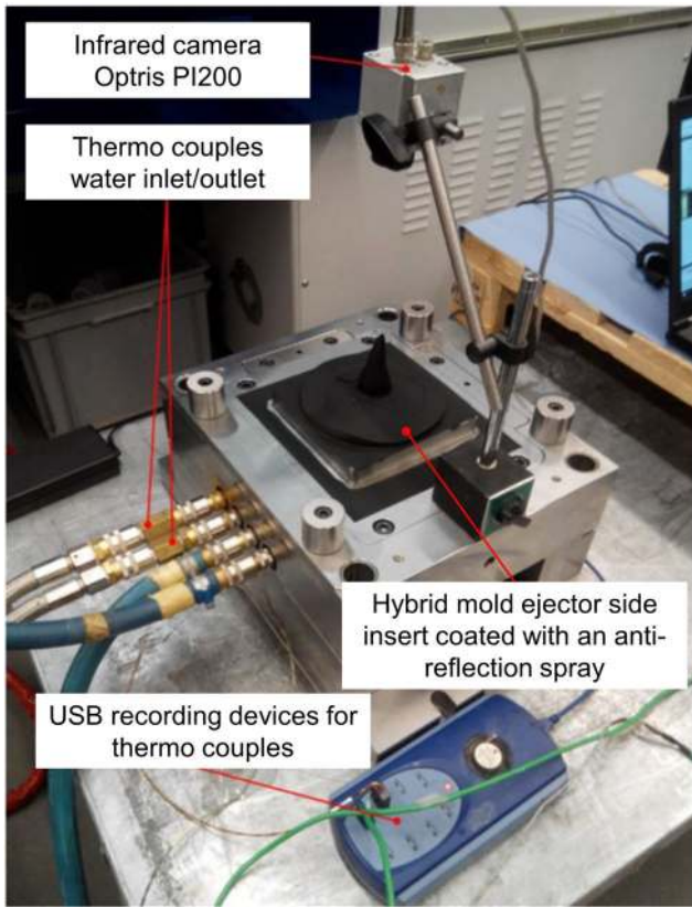
Fig. 12 Experimental setup
