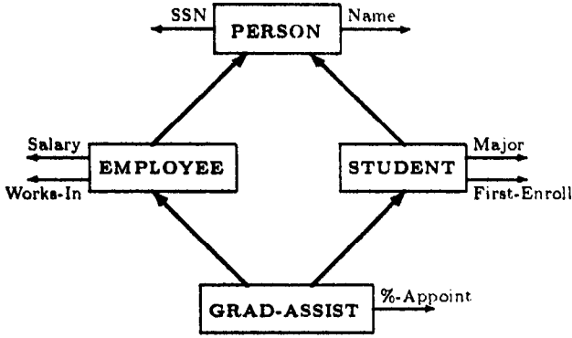
Figure 1: A Database Schema D
