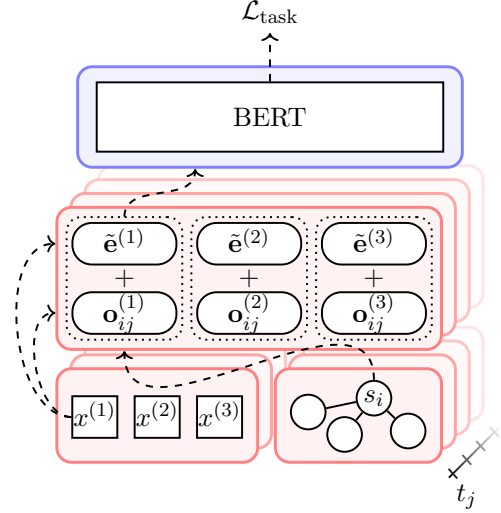
Figure 2: Model architecture. Words are mapped to dynamic embeddings by the parts of the dynamic component (red box), which are then contextualized by the contextualizer (blue box). The output of the contextualizer is used to compute the task-specific loss \mathcal{L}_{\text{task}} .
