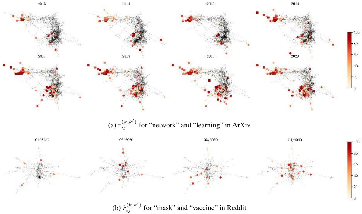
Figure 4: Spread of changes in the dominant sense through the social network. The figure shows dynamics in \hat{r}_{ij}^{(k,k')} , a score for semantic similarity between 0 (no similarity) and 100 (very similar), for “network” and “learning” in ArXiv as well as “mask” and “vaccine” in Reddit. The different node shapes in the ArXiv network represent the three major ArXiv subject classes: computer science (square), mathematics (triangle), and physics (circle). For “network”, the change towards the deep learning sense spread gradually from computer science and physics. For “mask”, the change towards the medical sense also spread gradually, with a major intensification after 03/2020.
