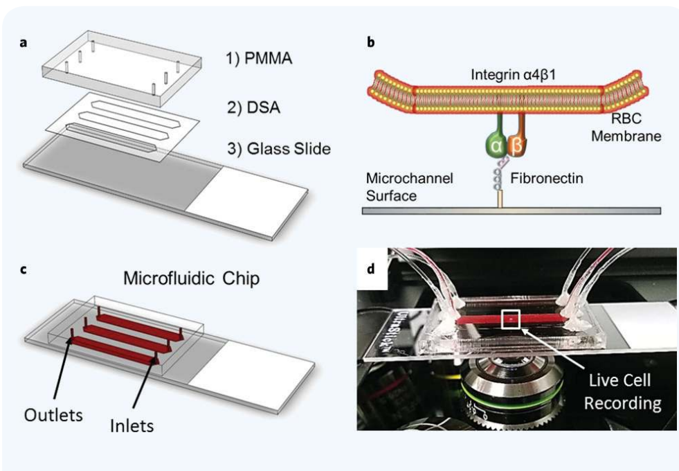
Figure 1 Microfluidic system for probing red blood cell (RBC) dynamic deformability. (a) Microfluidic system is composed of a poly(methyl methacrylate) (PMMA) cover, a double-sided adhesive (DSA) layer, which defines the channel shape and height (50 \mu\text{m} ) and a glass slide base. (b) Microfluidic channels are functionalized with fibronectin, which mimics the microvasculature wall in a closed system and can process whole blood. (c) PMMA top cover in the microfluidic system comprises micromachined inlets and outlets for tubing connections and blood injection. (d) Microfluidic system is placed on an automated microscope stage for live cell image recording.
