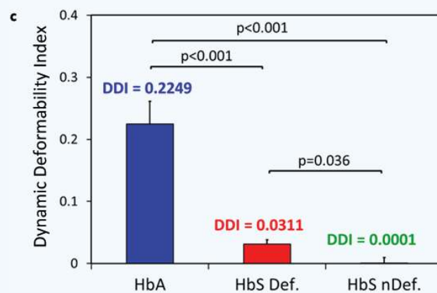
Figure 4 Dynamic deformability of healthy and sickle RBCs. (a) Dynamic deformability index (DDI) is determined as the rate of aspect ratio change in time in response to fluid shear stress. \text{DDI} = \tan(\alpha) , where \alpha is the angle between the change in CAR and the time of interest. (b) Healthy RBCs deformed at a much quicker rate and greater than non-deformable HbS and deformable HbS RBCs. Shown is the average curve for each group during deformation and the grey area indicates the time frame for when the HbA RBCs reached their deformed state. (c) The DDIs of each group were compared for the same amount of time (2 seconds, indicated by the grey area in b). The horizontal lines between individual groups represent statistically significant difference based on Kruskal-Wallis test followed by one-way ANOVA test with Fisher's post-hoc test for multiple comparisons ( n = 3-6 cells in a total of 12 blood samples; p < 0.05 ). Error bars represent standard error of the mean.
