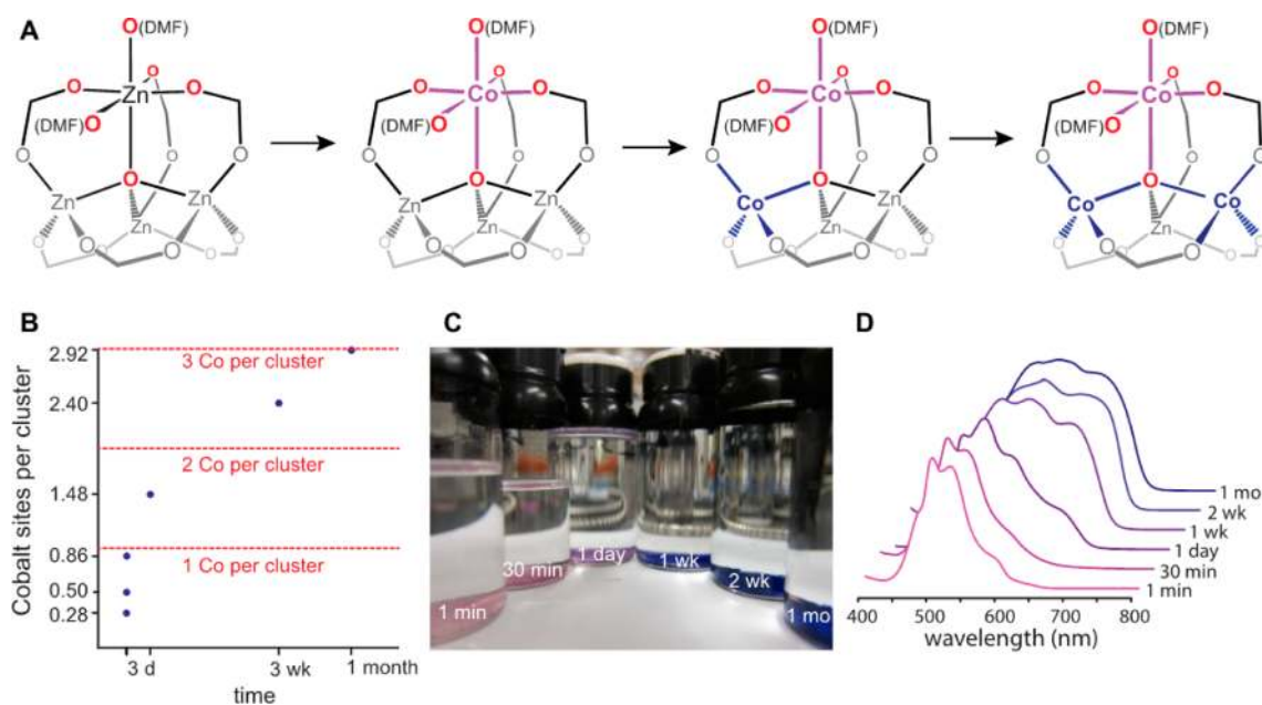
Figure 5. (A) The sequence of Co 2+ exchanges within the Zn_4O cluster of MOF-5, as suggested by the Co 2+ symmetry inferred from the UV–vis traces. (B) The results of ICP–AES analysis of MOF-5 soaked in CoCl 2 for periods between 1 min and 1 month. (C) Optical photographs of the Co–MOF-5 materials after cation exchange for periods denoted by the labels in white lettering. (D) Normalized diffused reflectance UV–visible traces of the various Co–MOF-5 materials with the length of cation exchange labeled by each trace.
