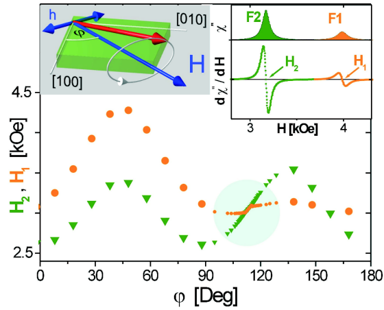
FIG. 1 (color online). Dependence of the FMR resonance fields H_1 (circles) and H_2 (triangles) for the thin Fe film F1 and the thick Fe film F2 , respectively, on the angle \varphi of the external dc magnetic field with respect to the Fe [100] crystallographic axis. The sketch of the in-plane magnetic measurement in the left inset shows how the rf magnetic field (double-pointed arrow) drives the magnetization (on a scale grossly exaggerated for easy viewing). In the right inset we plot the measured absorption peaks for layers F1 and F2 at \varphi = 60^\circ .
