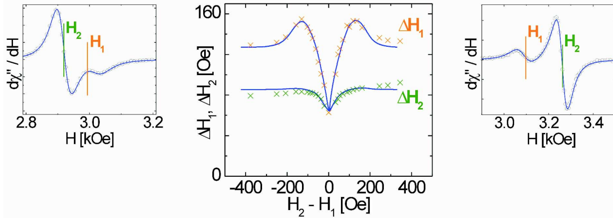
FIG. 3 (color online). Comparison of theory (solid lines) with RT measurements (symbols) close to and at the crossover of the FMR fields, marked by the shaded area in Fig. 1. The left and right frames show FMR signals for the field difference, H_2 - H_1 , of -78 Oe and +161 Oe, respectively. The theoretical results are parametrized by the full set of magnetic parameters which were measured independently [16]. The magnitude of the spin-pump current was determined by the linewidth at large separation of the FMR peaks. The middle frame displays the effective FMR linewidth of magnetic layers for the signals fitted by two Lorentzians as a function of the external field. At H_1 = H_2 , the FMR linewidths reached their minimum values at the level of intrinsic Gilbert damping of isolated films. The calculations in the middle frame did not take small variations of the intrinsic damping with angle \varphi into account, which resulted in deviations between theory and experiment for larger |H_1 - H_2| . Note that \Delta H_1 first increases before attaining its minimum, which is due to excitation of the antisymmetric collective mode.
