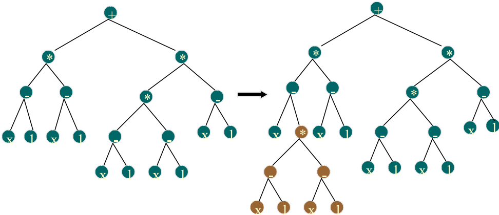
Figure 7. Example of expansion mutation
