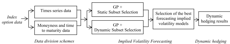
Figure 1. Description of the proposed approach's implementation
