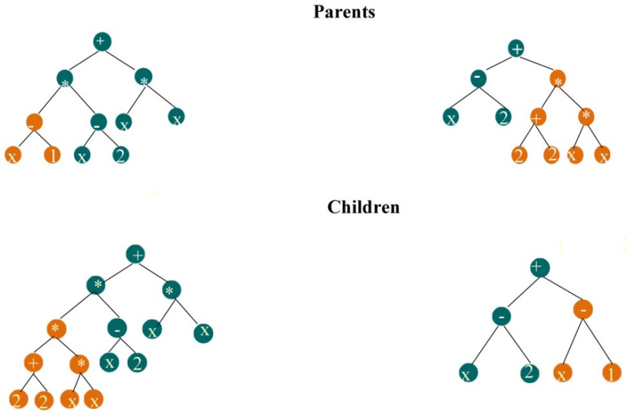
Figure 4. Example of subtree crossover
