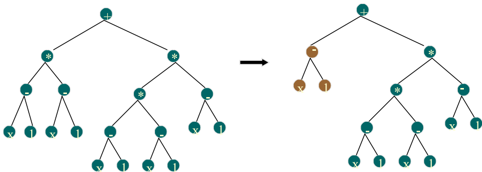
Figure 5. Example of subtree mutation
