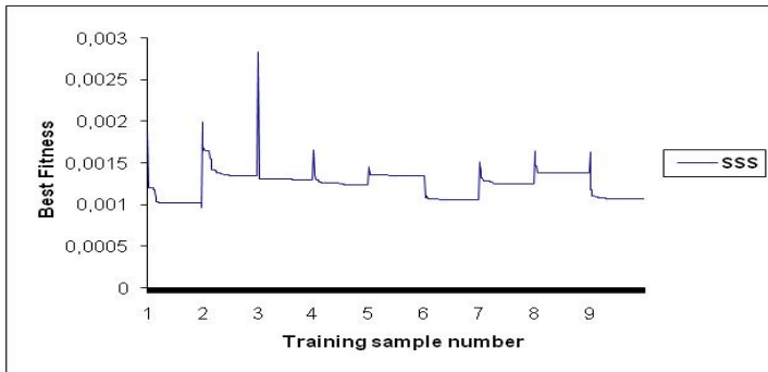
Figure 9. Example of curve fitness of the best individuals generated by genetic programming using SSS method for moneyness-time to maturity classes
