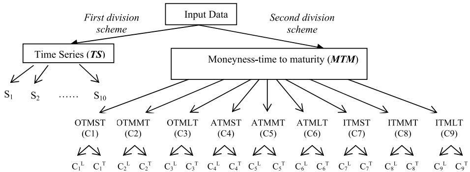
Figure 2. Data division schemes
